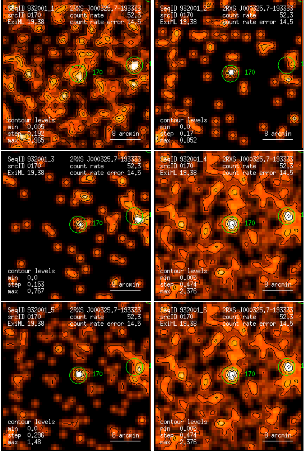
Figure 170: RASS 932001: detection 0170: band rate images, Gaussian filter: (1) PSPC channels 11 – 41, (2) 52 – 90, (3) 91 – 201, (4) 11 – 235, (5) 52 – 201, (6) 11 – 201. Broad band rates in counts/ks. Band rate contour levels in counts/ks/arcmin 2 .
