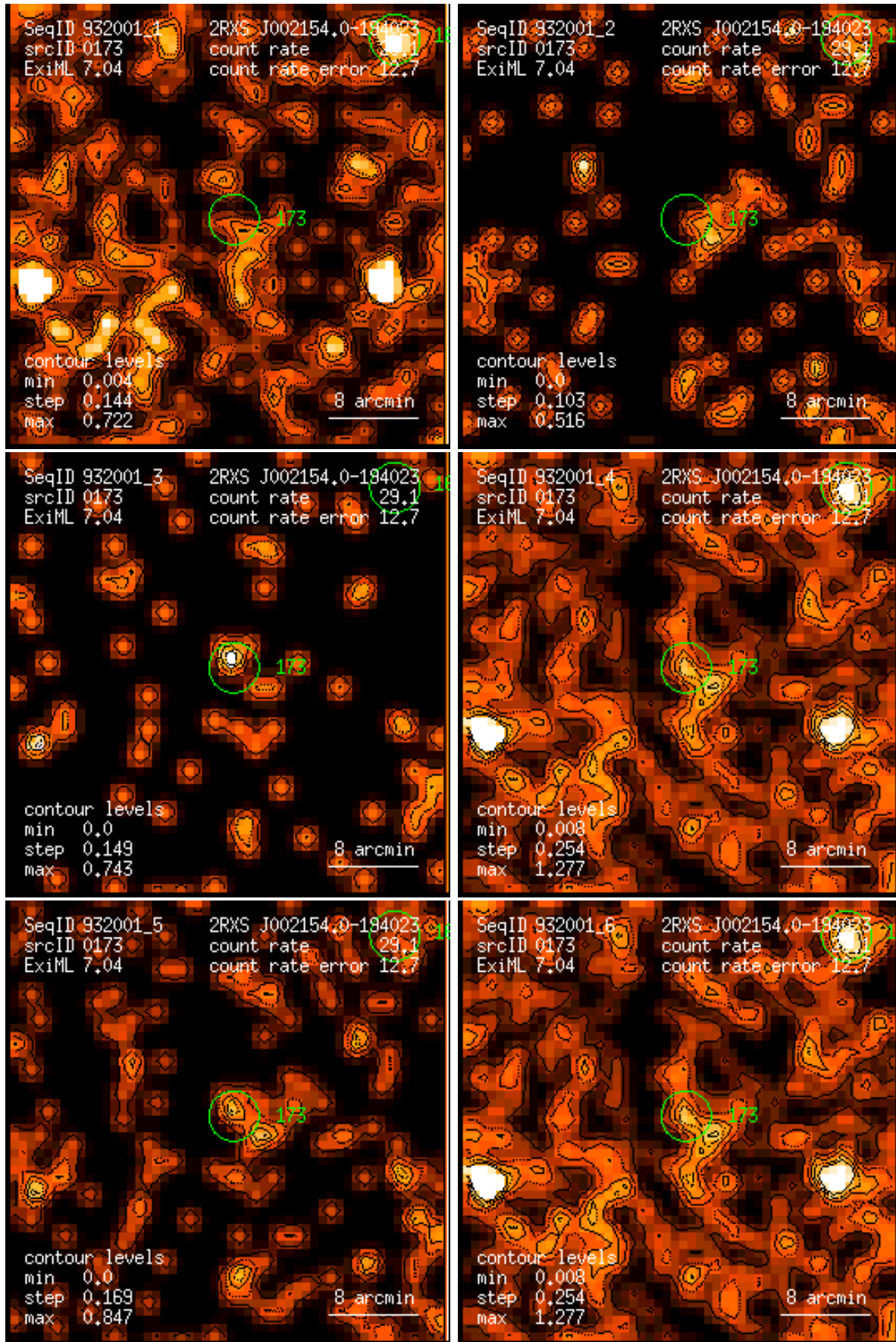
Figure 173: RASS 932001: detection 0173: band rate images, Gaussian filter: (1) PSPC channels 11 – 41, (2) 52 – 90, (3) 91 – 201, (4) 11 – 235, (5) 52 – 201, (6) 11 – 201. Broad band rates in counts/ks. Band rate contour levels in counts/ks/arcmin 2 .
