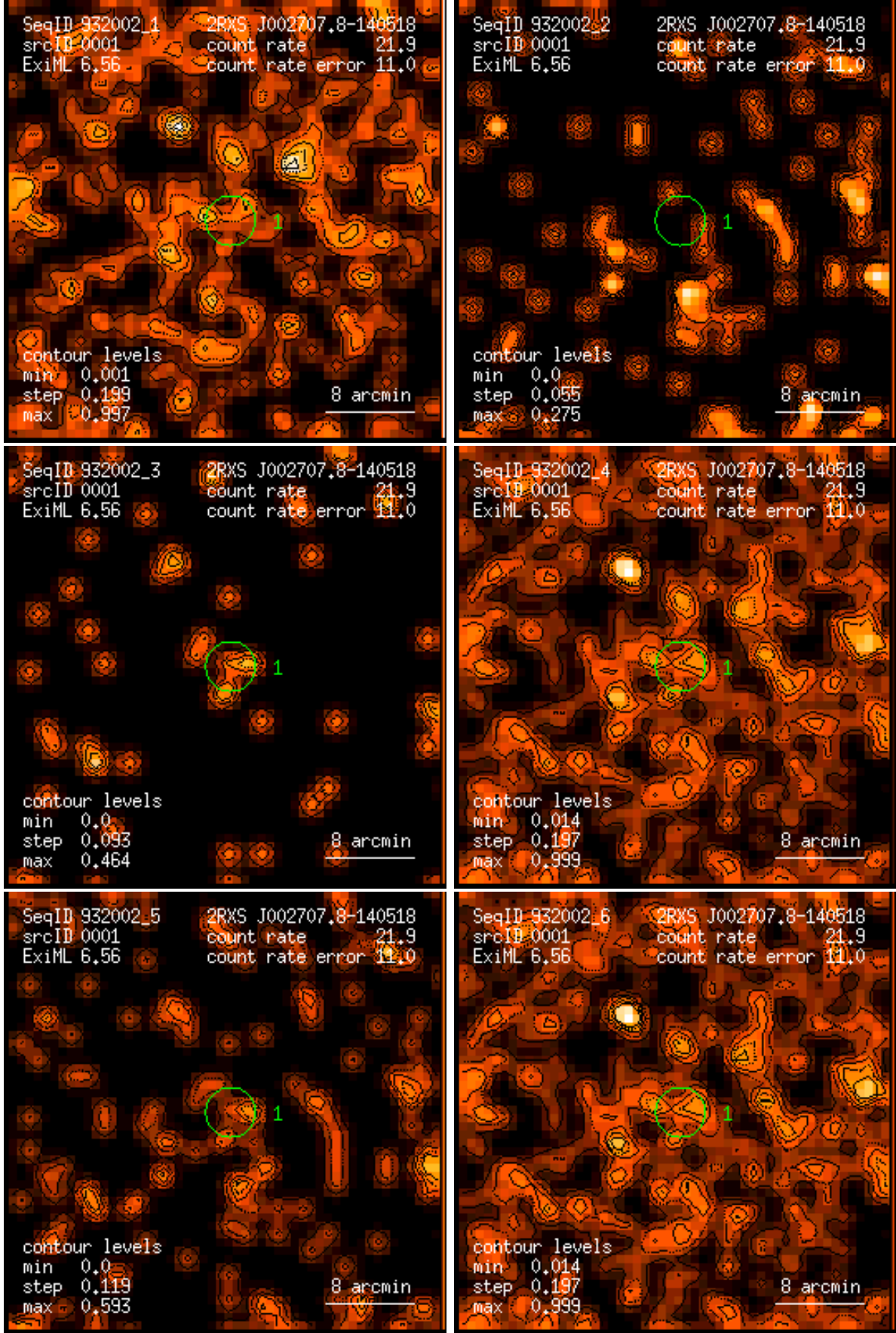
Figure 1: RASS 932002: detection 0001: band rate images, Gaussian filter: (1) PSPC channels 11 – 41, (2) 52 – 90, (3) 91 – 201, (4) 11 – 235, (5) 52 – 201, (6) 11 – 201. Broad band rates in counts/ks. Band rate contour levels in counts/ks/arcmin 2 .
