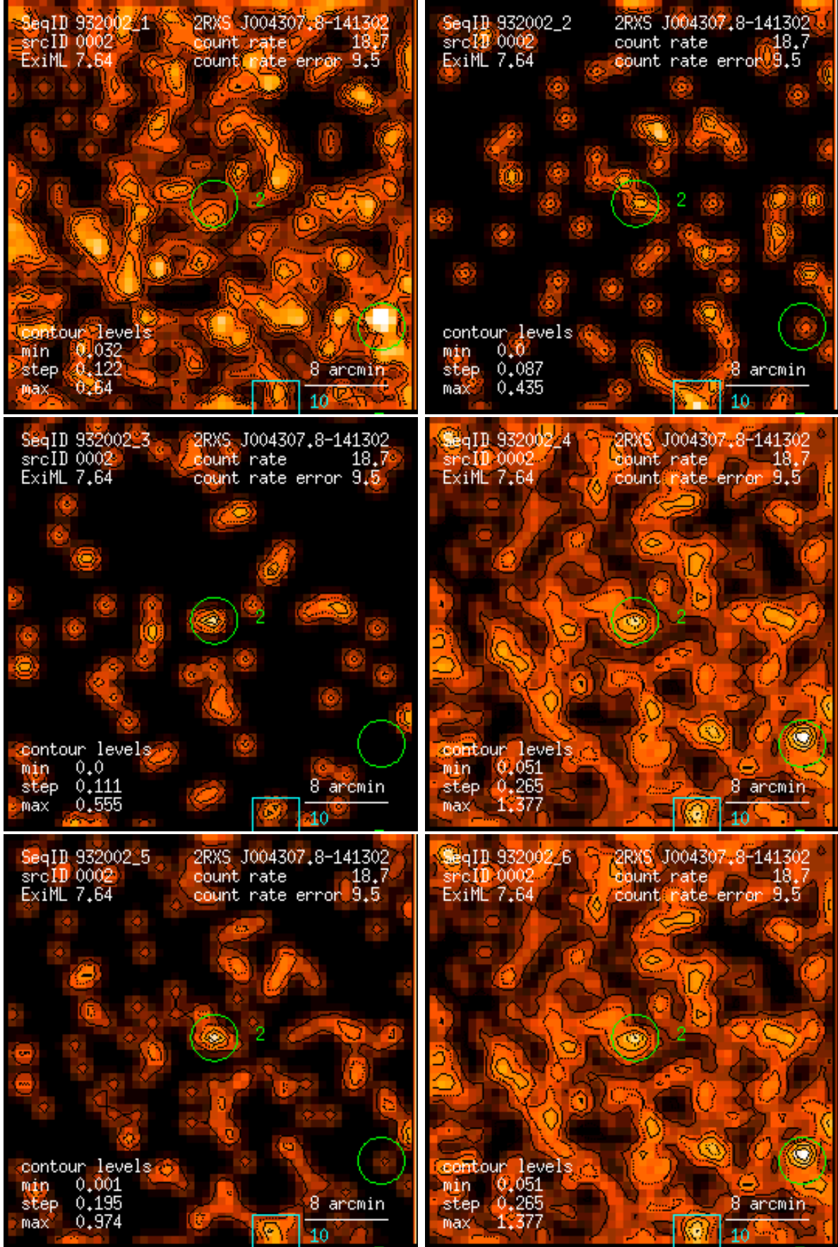
Figure 2: RASS 932002: detection 0002: band rate images, Gaussian filter: (1) PSPC channels 11 – 41, (2) 52 – 90, (3) 91 – 201, (4) 11 – 235, (5) 52 – 201, (6) 11 – 201. Broad band rates in counts/ks. Band rate contour levels in counts/ks/arcmin 2 .
