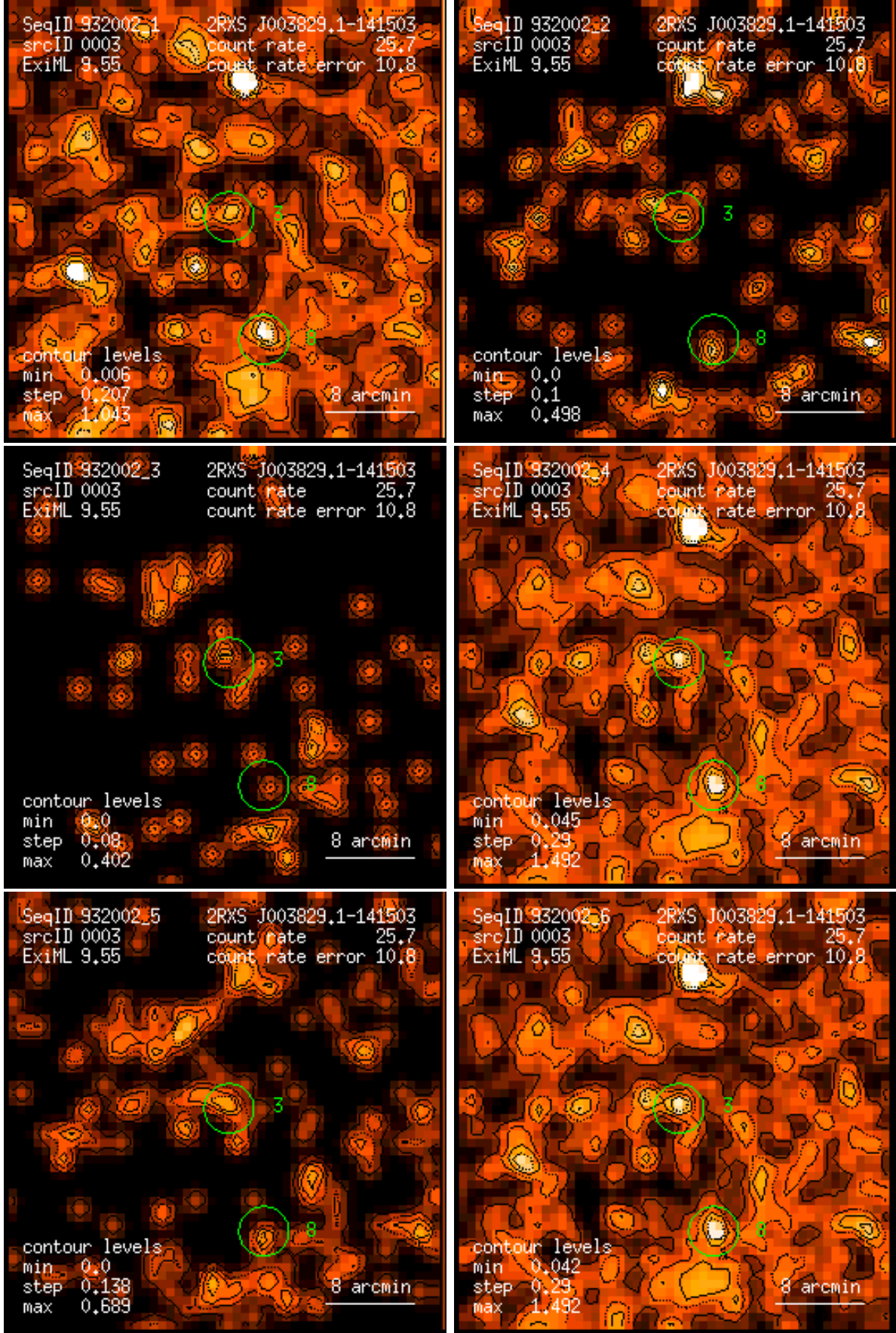
Figure 3: RASS 932002: detection 0003: band rate images, Gaussian filter: (1) PSPC channels 11 – 41, (2) 52 – 90, (3) 91 – 201, (4) 11 – 235, (5) 52 – 201, (6) 11 – 201. Broad band rates in counts/ks. Band rate contour levels in counts/ks/arcmin 2 .
