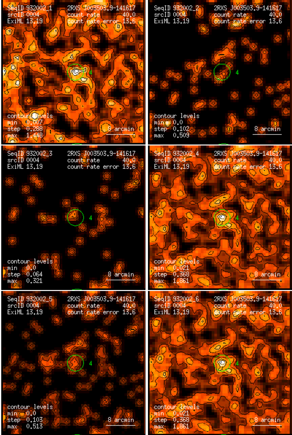
Figure 4: RASS 932002: detection 0004: band rate images, Gaussian filter: (1) PSPC channels 11 – 41, (2) 52 – 90, (3) 91 – 201, (4) 11 – 235, (5) 52 – 201, (6) 11 – 201. Broad band rates in counts/ks. Band rate contour levels in counts/ks/arcmin 2 .
