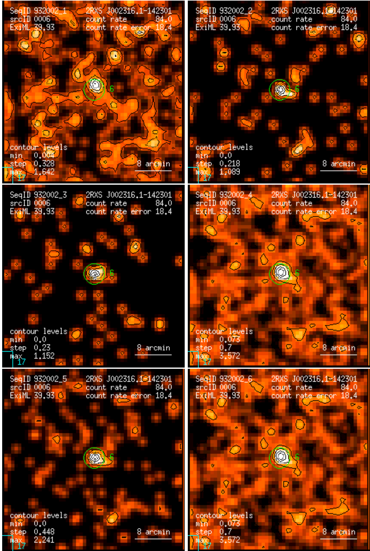
Figure 6: RASS 932002: detection 0006: band rate images, Gaussian filter: (1) PSPC channels 11 – 41, (2) 52 – 90, (3) 91 – 201, (4) 11 – 235, (5) 52 – 201, (6) 11 – 201. Broad band rates in counts/ks. Band rate contour levels in counts/ks/arcmin 2 .
