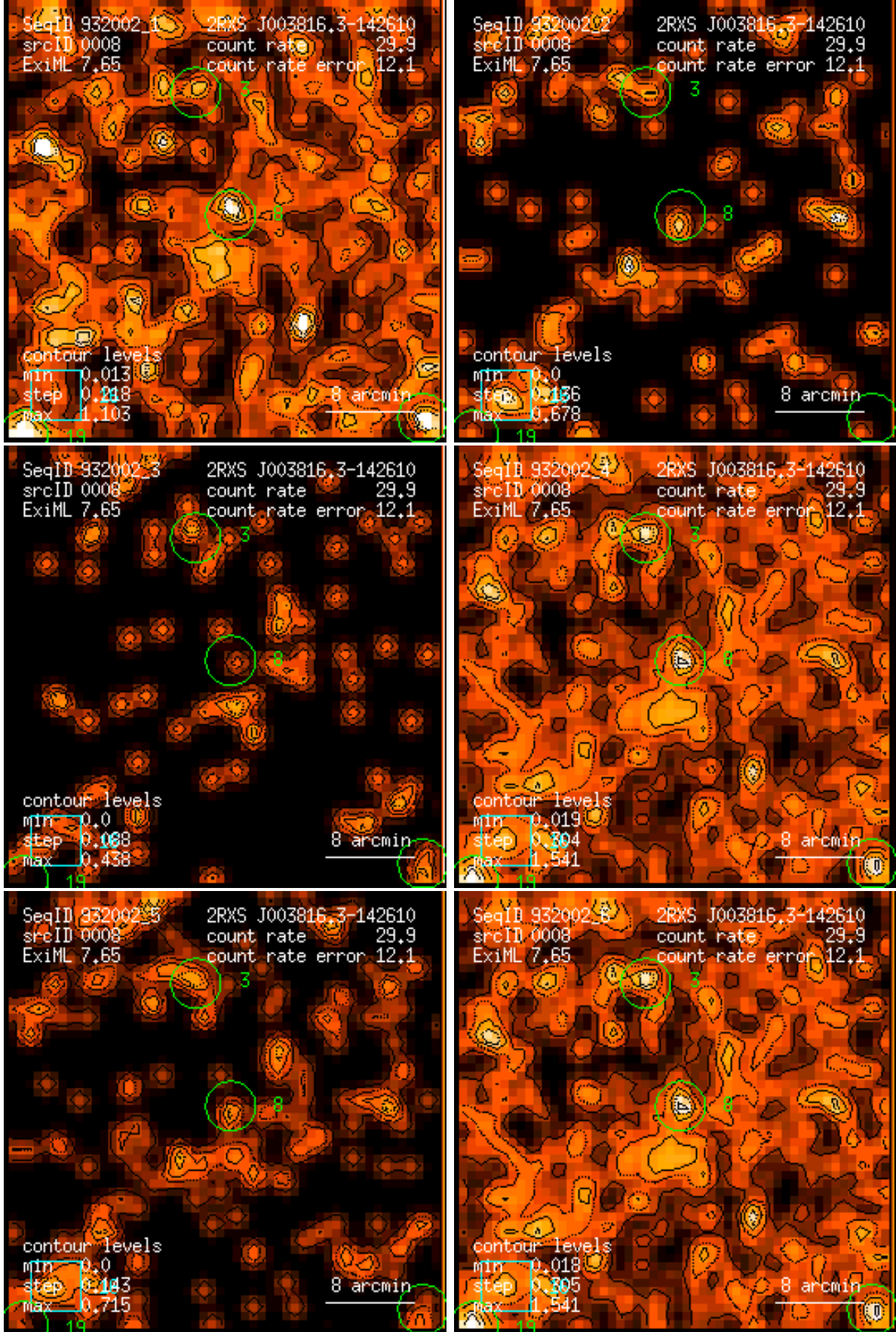
Figure 8: RASS 932002: detection 0008: band rate images, Gaussian filter: (1) PSPC channels 11 – 41, (2) 52 – 90, (3) 91 – 201, (4) 11 – 235, (5) 52 – 201, (6) 11 – 201. Broad band rates in counts/ks. Band rate contour levels in counts/ks/arcmin 2 .
