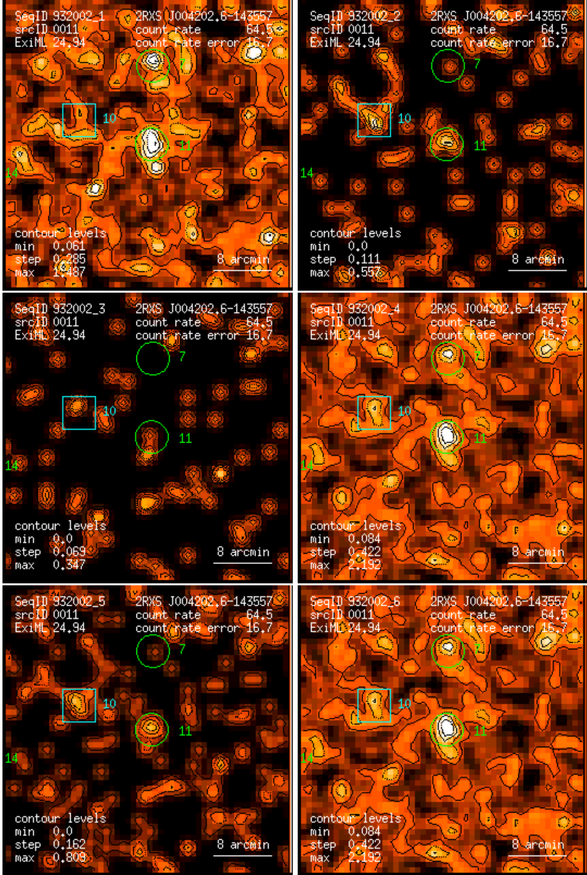
Figure 11: RASS 932002: detection 0011: band rate images, Gaussian filter: (1) PSPC channels 11 – 41, (2) 52 – 90, (3) 91 – 201, (4) 11 – 235, (5) 52 – 201, (6) 11 – 201. Broad band rates in counts/ks. Band rate contour levels in counts/ks/arcmin 2 .
