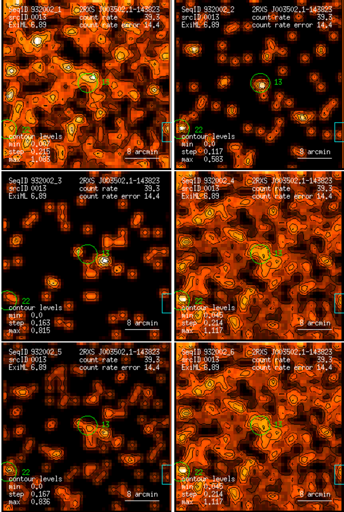
Figure 13: RASS 932002: detection 0013: band rate images, Gaussian filter: (1) PSPC channels 11 – 41, (2) 52 – 90, (3) 91 – 201, (4) 11 – 235, (5) 52 – 201, (6) 11 – 201. Broad band rates in counts/ks. Band rate contour levels in counts/ks/arcmin 2 .
