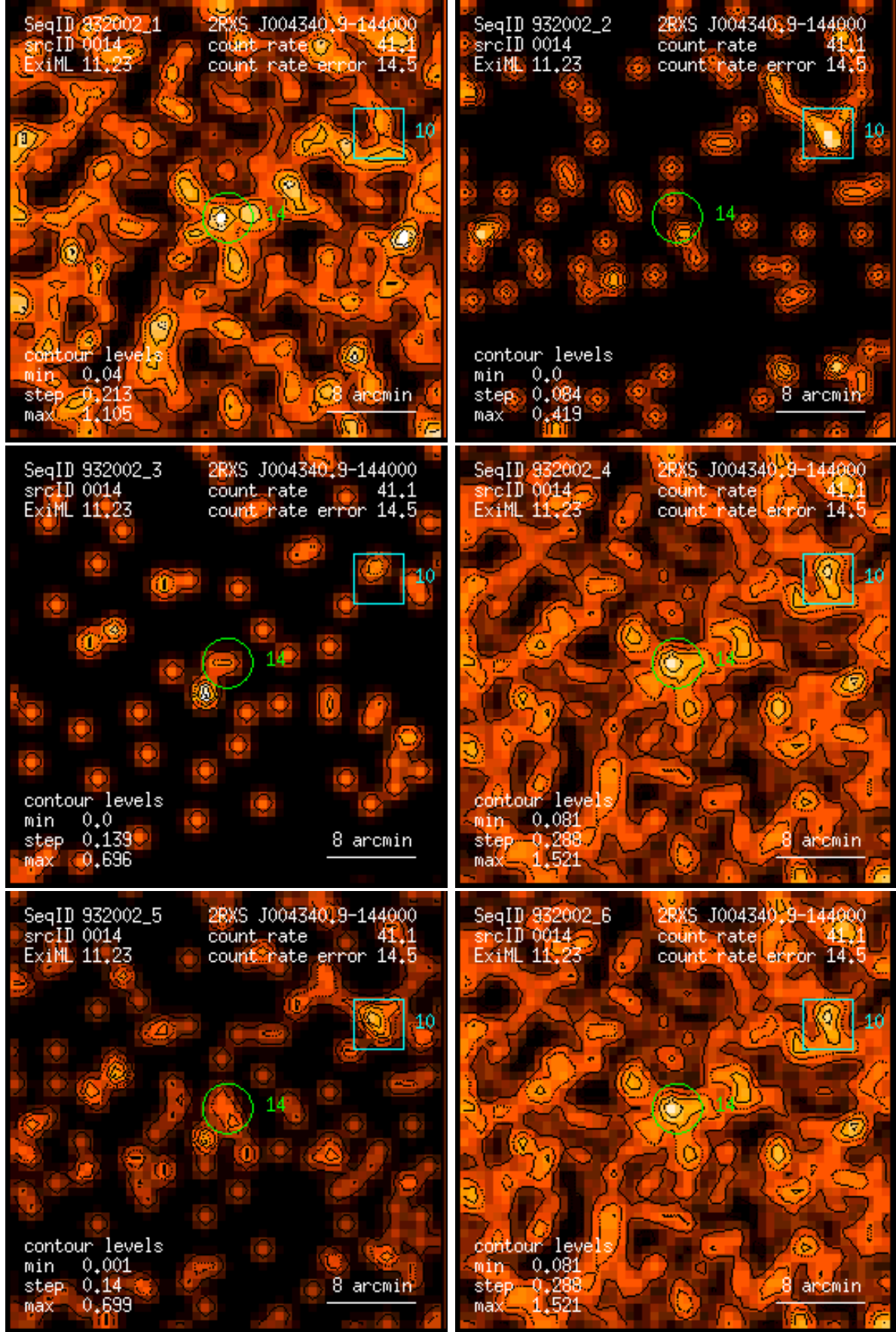
Figure 14: RASS 932002: detection 0014: band rate images, Gaussian filter: (1) PSPC channels 11 – 41, (2) 52 – 90, (3) 91 – 201, (4) 11 – 235, (5) 52 – 201, (6) 11 – 201. Broad band rates in counts/ks. Band rate contour levels in counts/ks/arcmin 2 .
