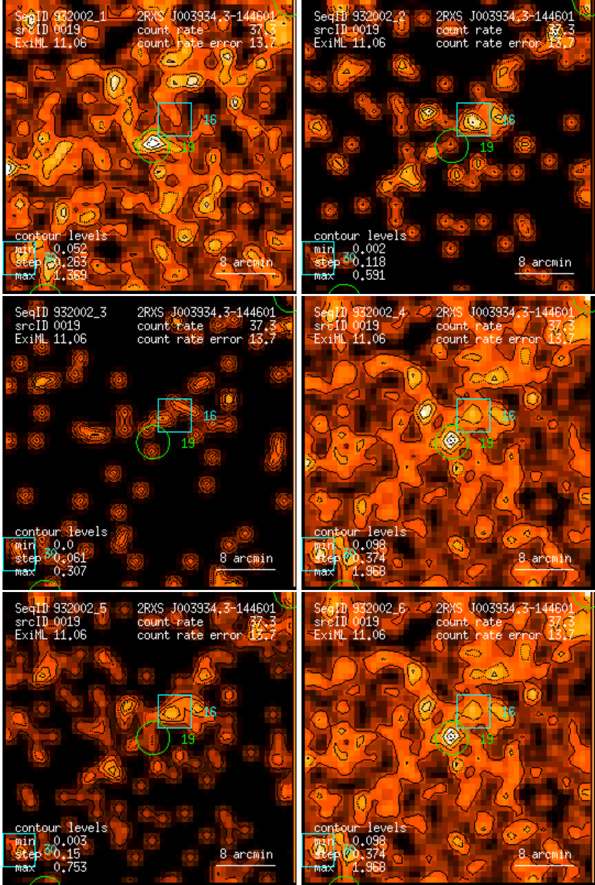
Figure 19: RASS 932002: detection 0019: band rate images, Gaussian filter: (1) PSPC channels 11 – 41, (2) 52 – 90, (3) 91 – 201, (4) 11 – 235, (5) 52 – 201, (6) 11 – 201. Broad band rates in counts/ks. Band rate contour levels in counts/ks/arcmin 2 .
