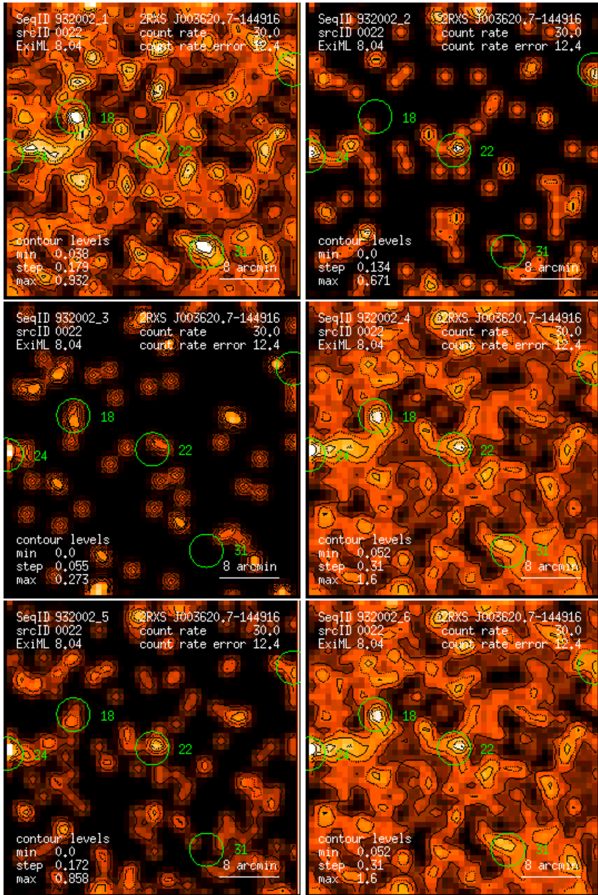
Figure 22: RASS 932002: detection 0022: band rate images, Gaussian filter: (1) PSPC channels 11 – 41, (2) 52 – 90, (3) 91 – 201, (4) 11 – 235, (5) 52 – 201, (6) 11 – 201. Broad band rates in counts/ks. Band rate contour levels in counts/ks/arcmin 2 .
