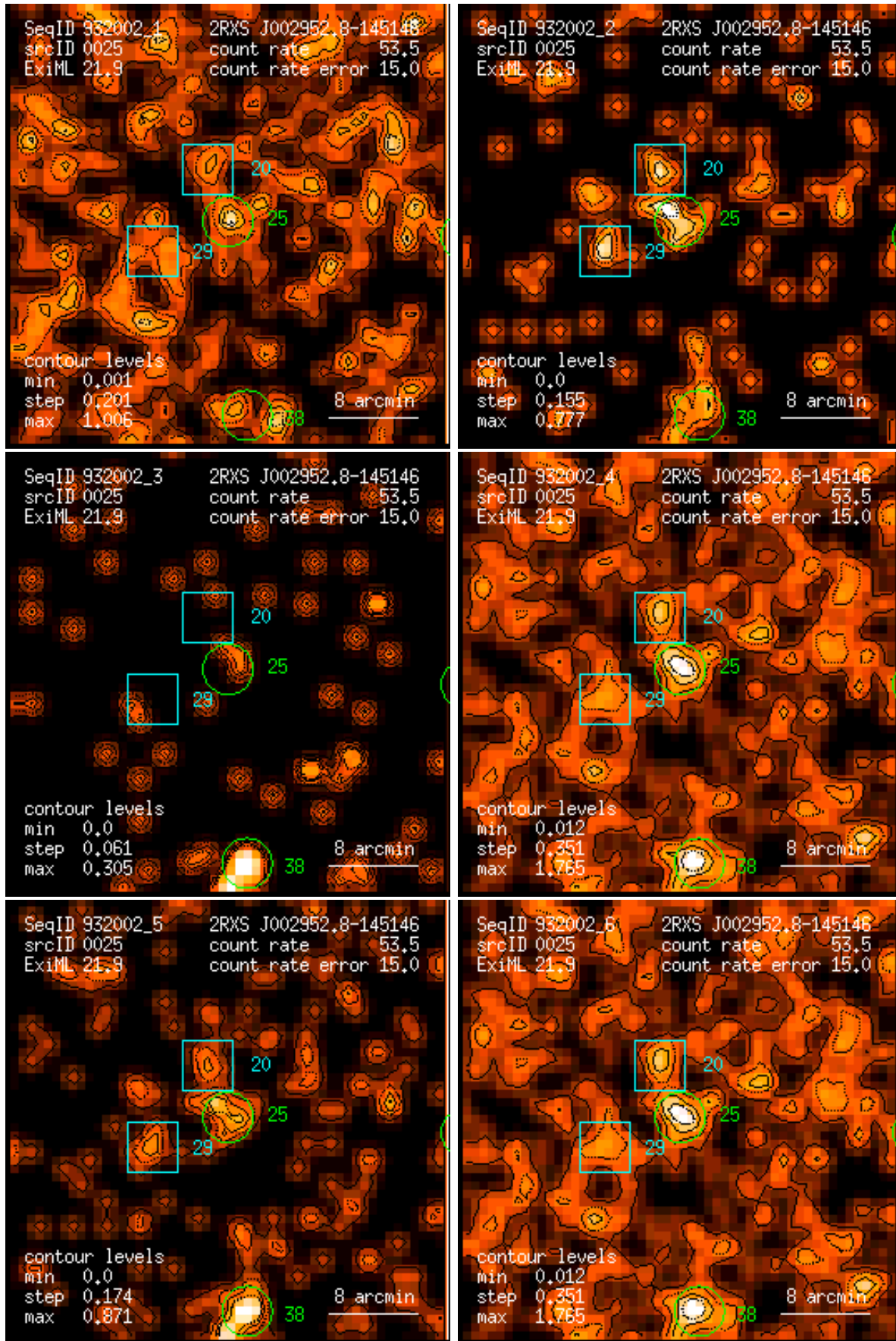
Figure 25: RASS 932002: detection 0025: band rate images, Gaussian filter: (1) PSPC channels 11 – 41, (2) 52 – 90, (3) 91 – 201, (4) 11 – 235, (5) 52 – 201, (6) 11 – 201. Broad band rates in counts/ks. Band rate contour levels in counts/ks/arcmin 2 .
