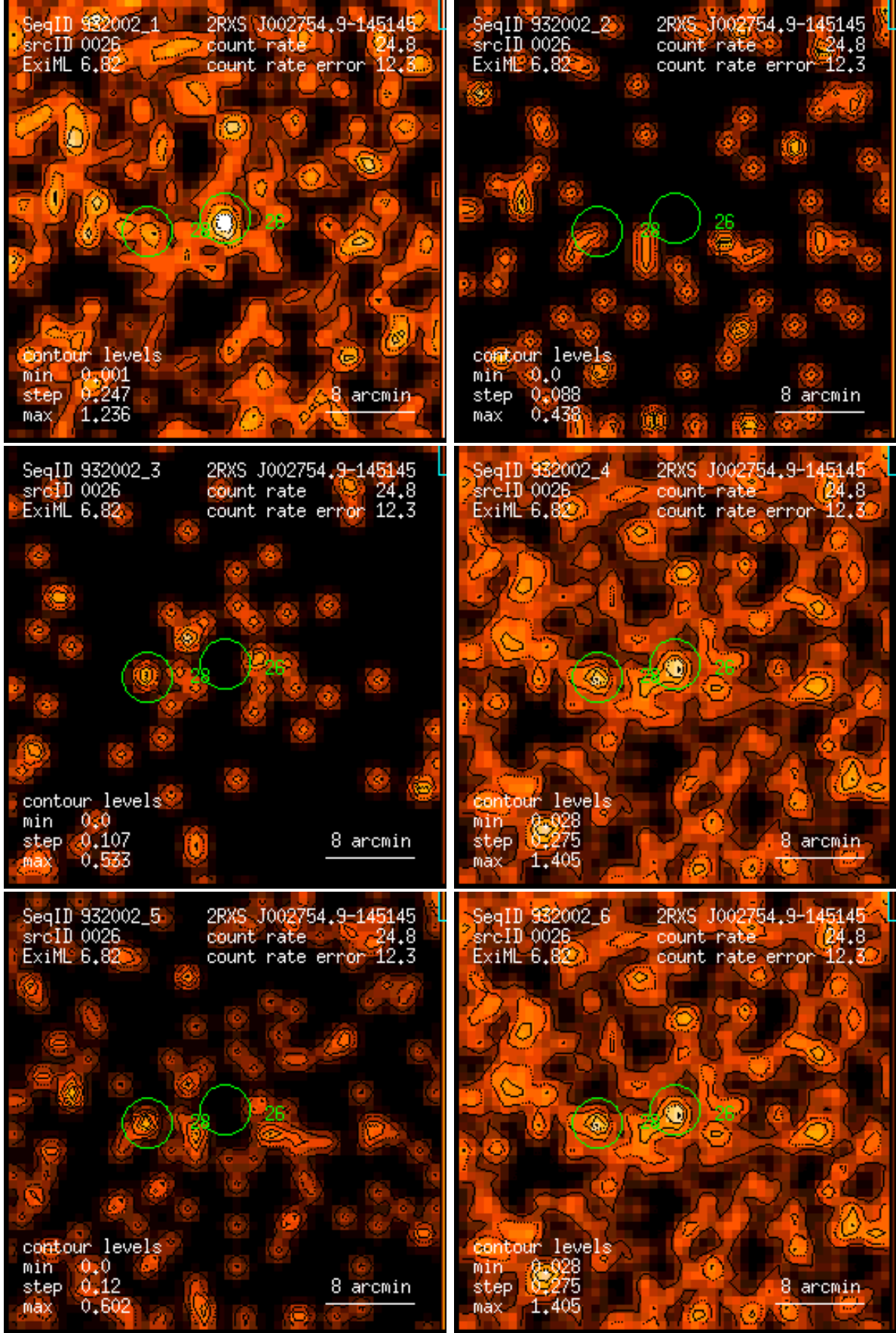
Figure 26: RASS 932002: detection 0026: band rate images, Gaussian filter: (1) PSPC channels 11 – 41, (2) 52 – 90, (3) 91 – 201, (4) 11 – 235, (5) 52 – 201, (6) 11 – 201. Broad band rates in counts/ks. Band rate contour levels in counts/ks/arcmin 2 .
