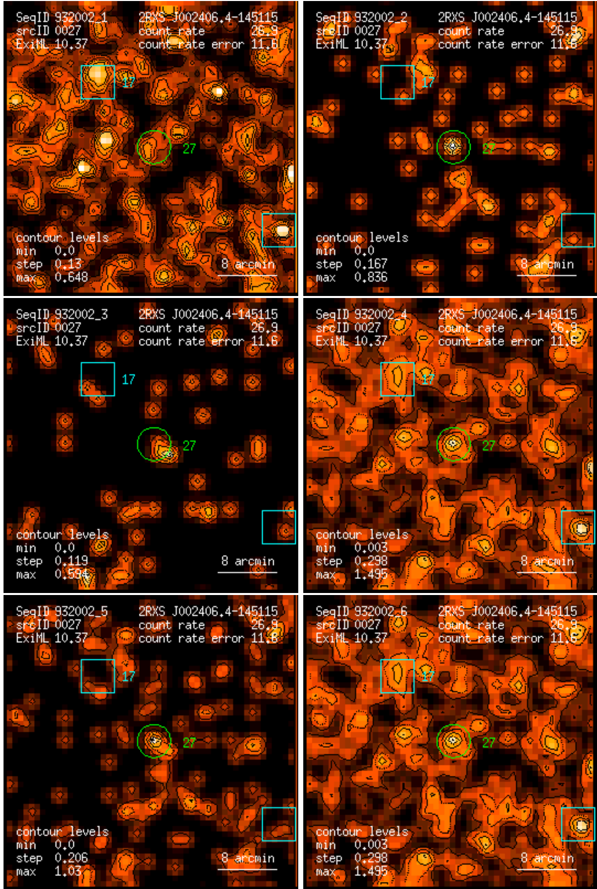
Figure 27: RASS 932002: detection 0027: band rate images, Gaussian filter: (1) PSPC channels 11 – 41, (2) 52 – 90, (3) 91 – 201, (4) 11 – 235, (5) 52 – 201, (6) 11 – 201. Broad band rates in counts/ks. Band rate contour levels in counts/ks/arcmin 2 .
