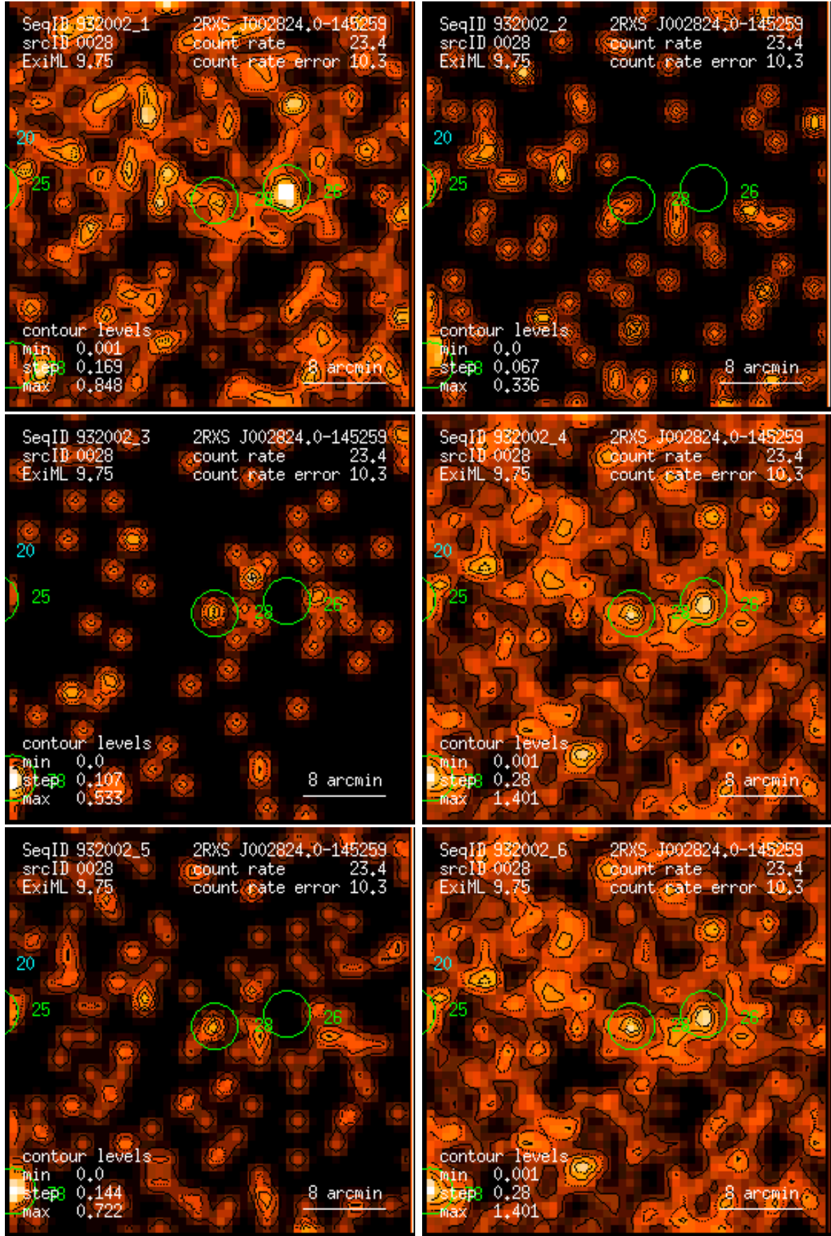
Figure 28: RASS 932002: detection 0028: band rate images, Gaussian filter: (1) PSPC channels 11 – 41, (2) 52 – 90, (3) 91 – 201, (4) 11 – 235, (5) 52 – 201, (6) 11 – 201. Broad band rates in counts/ks. Band rate contour levels in counts/ks/arcmin 2 .
