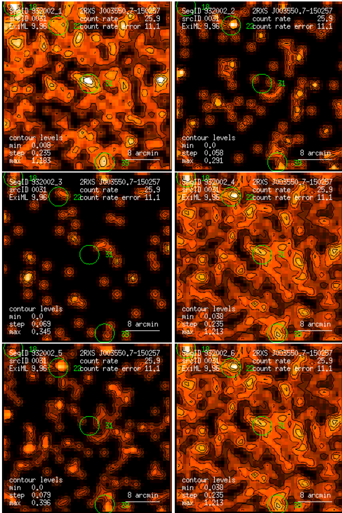
Figure 31: RASS 932002: detection 0031: band rate images, Gaussian filter: (1) PSPC channels 11 – 41, (2) 52 – 90, (3) 91 – 201, (4) 11 – 235, (5) 52 – 201, (6) 11 – 201. Broad band rates in counts/ks. Band rate contour levels in counts/ks/arcmin 2 .
