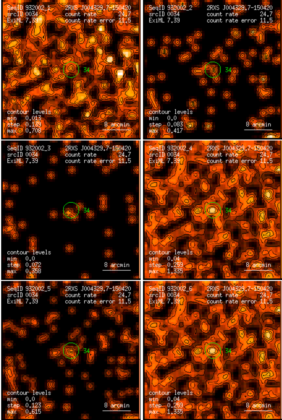
Figure 34: RASS 932002: detection 0034: band rate images, Gaussian filter: (1) PSPC channels 11 – 41, (2) 52 – 90, (3) 91 – 201, (4) 11 – 235, (5) 52 – 201, (6) 11 – 201. Broad band rates in counts/ks. Band rate contour levels in counts/ks/arcmin 2 .
