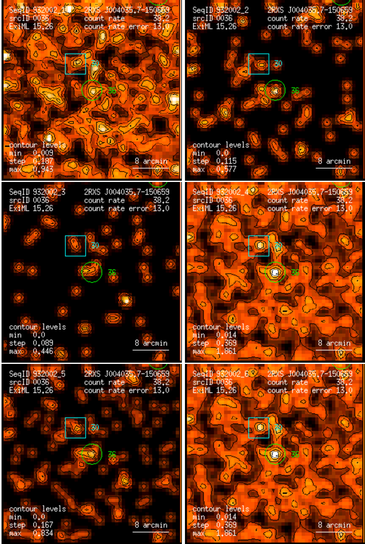
Figure 36: RASS 932002: detection 0036: band rate images, Gaussian filter: (1) PSPC channels 11 – 41, (2) 52 – 90, (3) 91 – 201, (4) 11 – 235, (5) 52 – 201, (6) 11 – 201. Broad band rates in counts/ks. Band rate contour levels in counts/ks/arcmin 2 .
