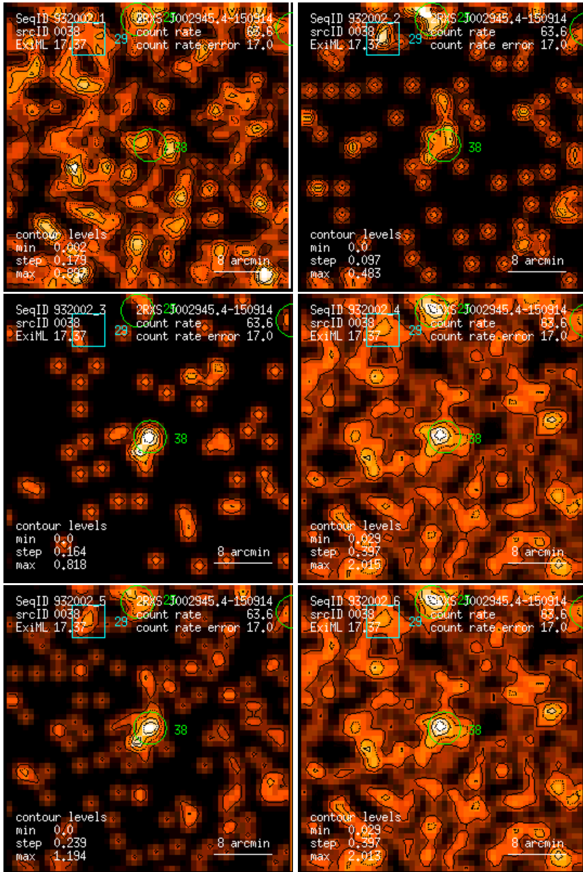
Figure 38: RASS 932002: detection 0038: band rate images, Gaussian filter: (1) PSPC channels 11 – 41, (2) 52 – 90, (3) 91 – 201, (4) 11 – 235, (5) 52 – 201, (6) 11 – 201. Broad band rates in counts/ks. Band rate contour levels in counts/ks/arcmin 2 .
