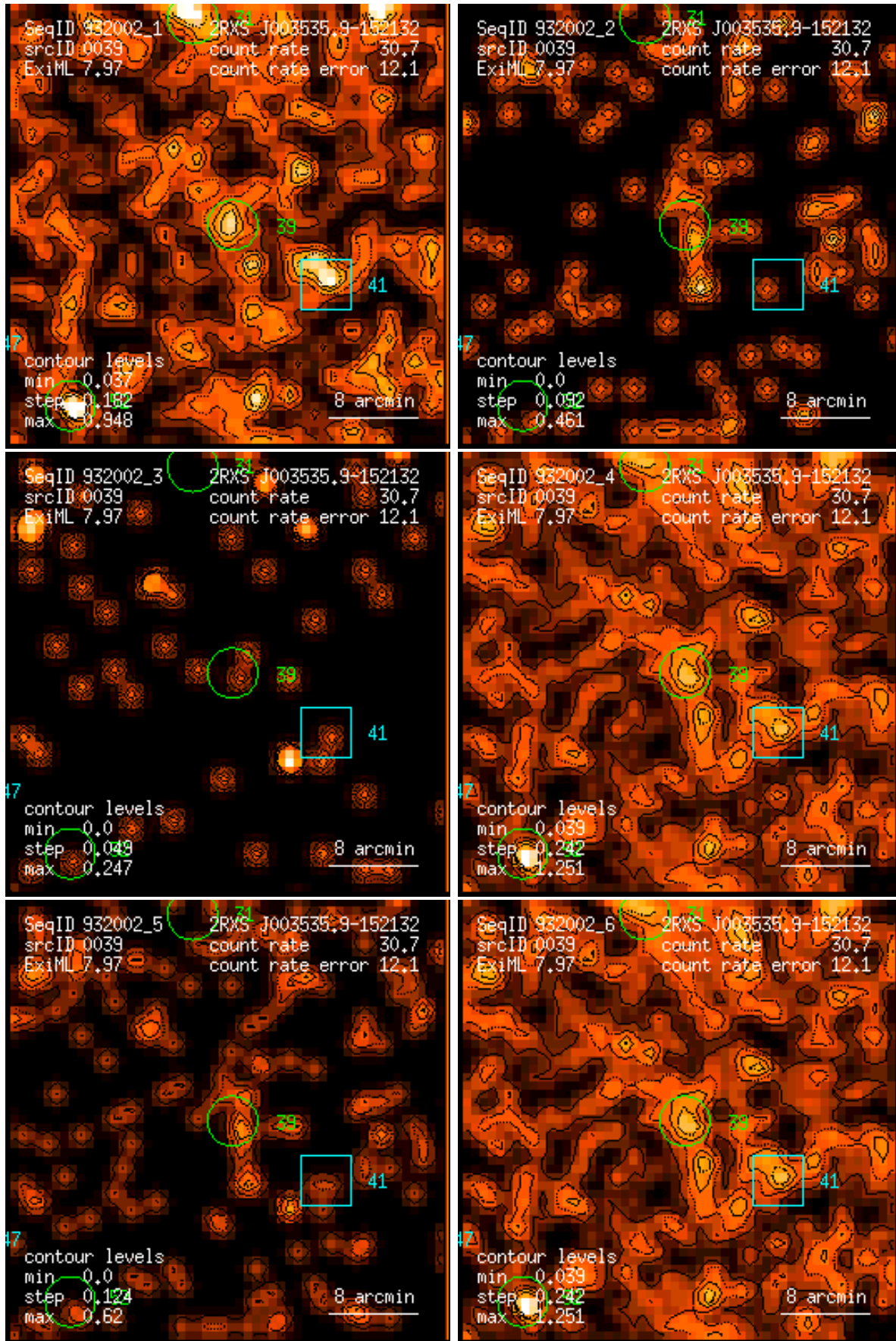
Figure 39: RASS 932002: detection 0039: band rate images, Gaussian filter: (1) PSPC channels 11 – 41, (2) 52 – 90, (3) 91 – 201, (4) 11 – 235, (5) 52 – 201, (6) 11 – 201. Broad band rates in counts/ks. Band rate contour levels in counts/ks/arcmin 2 .
