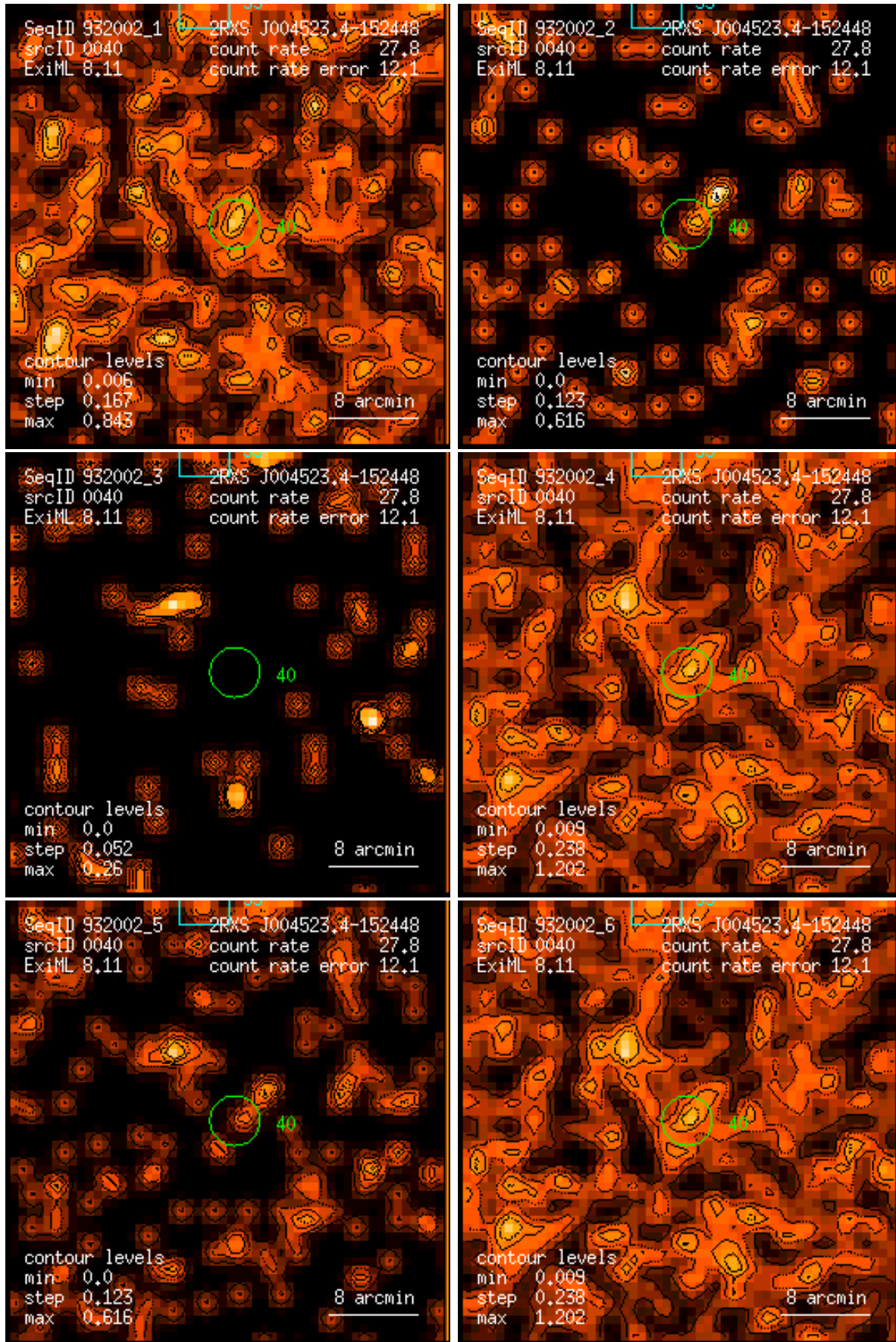
Figure 40: RASS 932002: detection 0040: band rate images, Gaussian filter: (1) PSPC channels 11 – 41, (2) 52 – 90, (3) 91 – 201, (4) 11 – 235, (5) 52 – 201, (6) 11 – 201. Broad band rates in counts/ks. Band rate contour levels in counts/ks/arcmin 2 .
