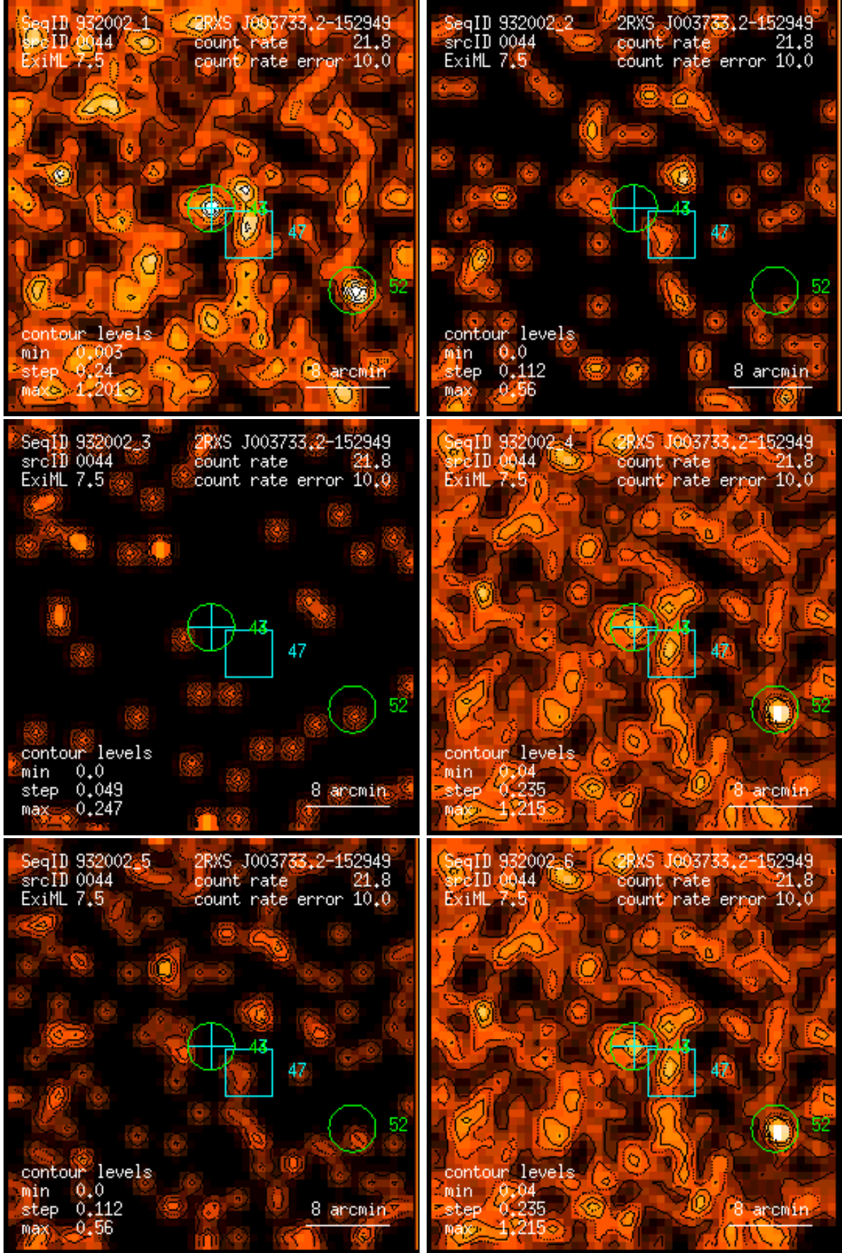
Figure 44: RASS 932002: detection 0044: band rate images, Gaussian filter: (1) PSPC channels 11 – 41, (2) 52 – 90, (3) 91 – 201, (4) 11 – 235, (5) 52 – 201, (6) 11 – 201. Broad band rates in counts/ks. Band rate contour levels in counts/ks/arcmin 2 .
