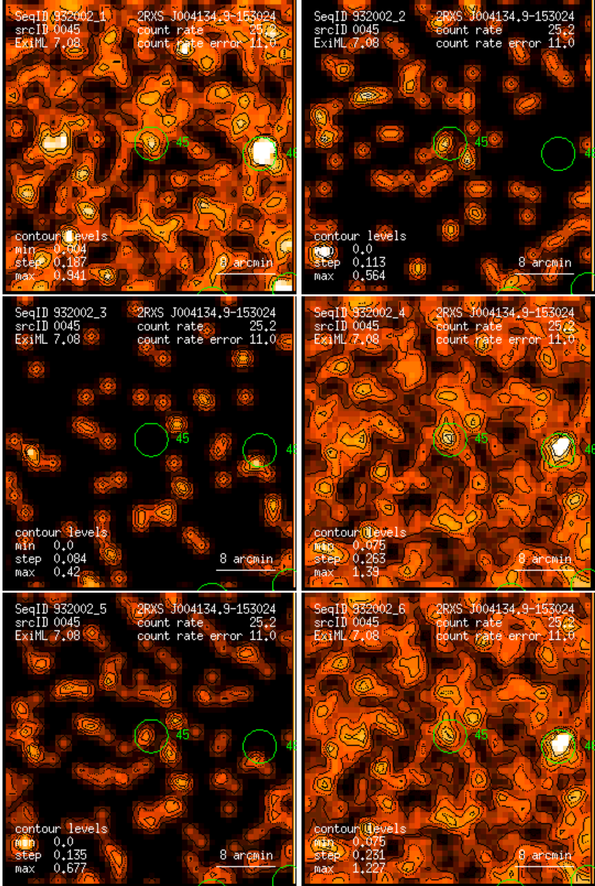
Figure 45: RASS 932002: detection 0045: band rate images, Gaussian filter: (1) PSPC channels 11 – 41, (2) 52 – 90, (3) 91 – 201, (4) 11 – 235, (5) 52 – 201, (6) 11 – 201. Broad band rates in counts/ks. Band rate contour levels in counts/ks/arcmin 2 .
