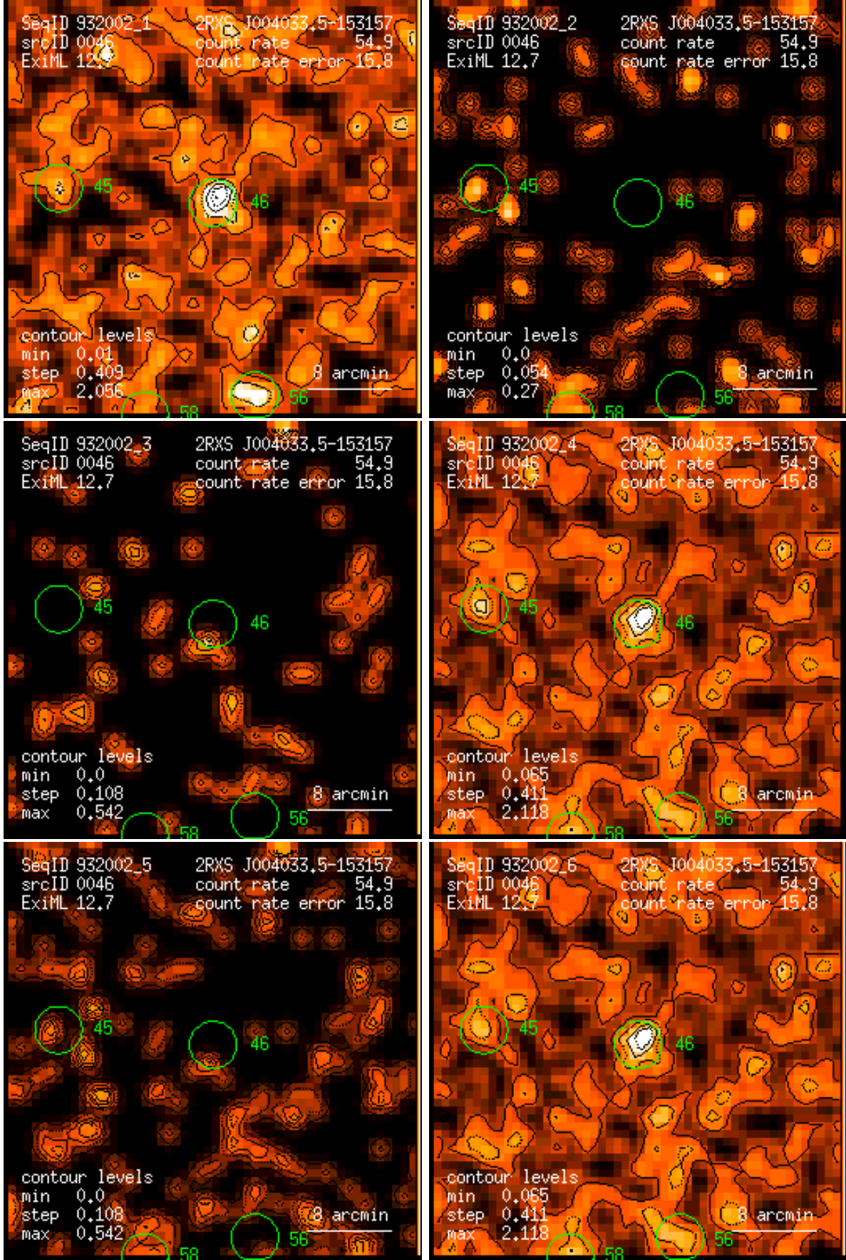
Figure 46: RASS 932002: detection 0046: band rate images, Gaussian filter: (1) PSPC channels 11 – 41, (2) 52 – 90, (3) 91 – 201, (4) 11 – 235, (5) 52 – 201, (6) 11 – 201. Broad band rates in counts/ks. Band rate contour levels in counts/ks/arcmin 2 .
