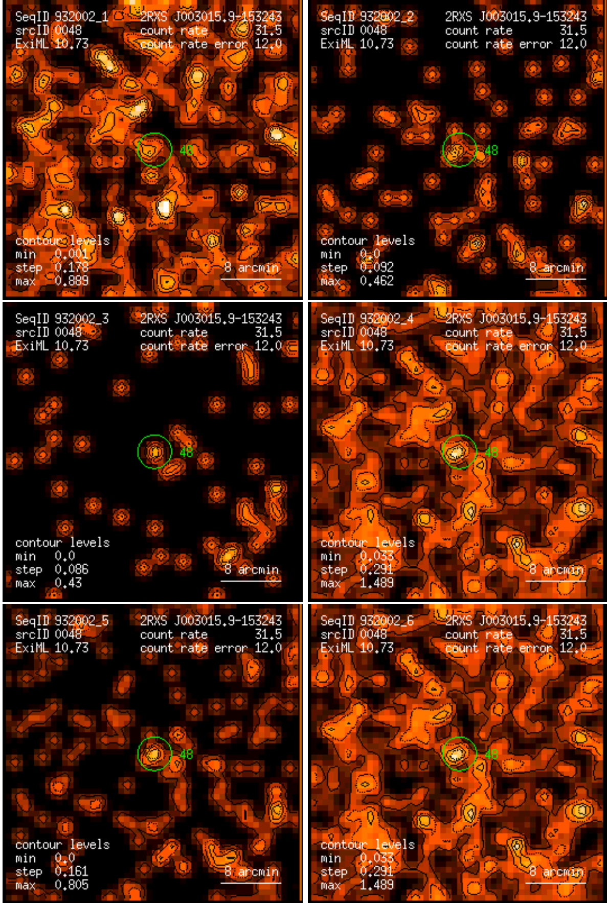
Figure 48: RASS 932002: detection 0048: band rate images, Gaussian filter: (1) PSPC channels 11 – 41, (2) 52 – 90, (3) 91 – 201, (4) 11 – 235, (5) 52 – 201, (6) 11 – 201. Broad band rates in counts/ks. Band rate contour levels in counts/ks/arcmin 2 .
