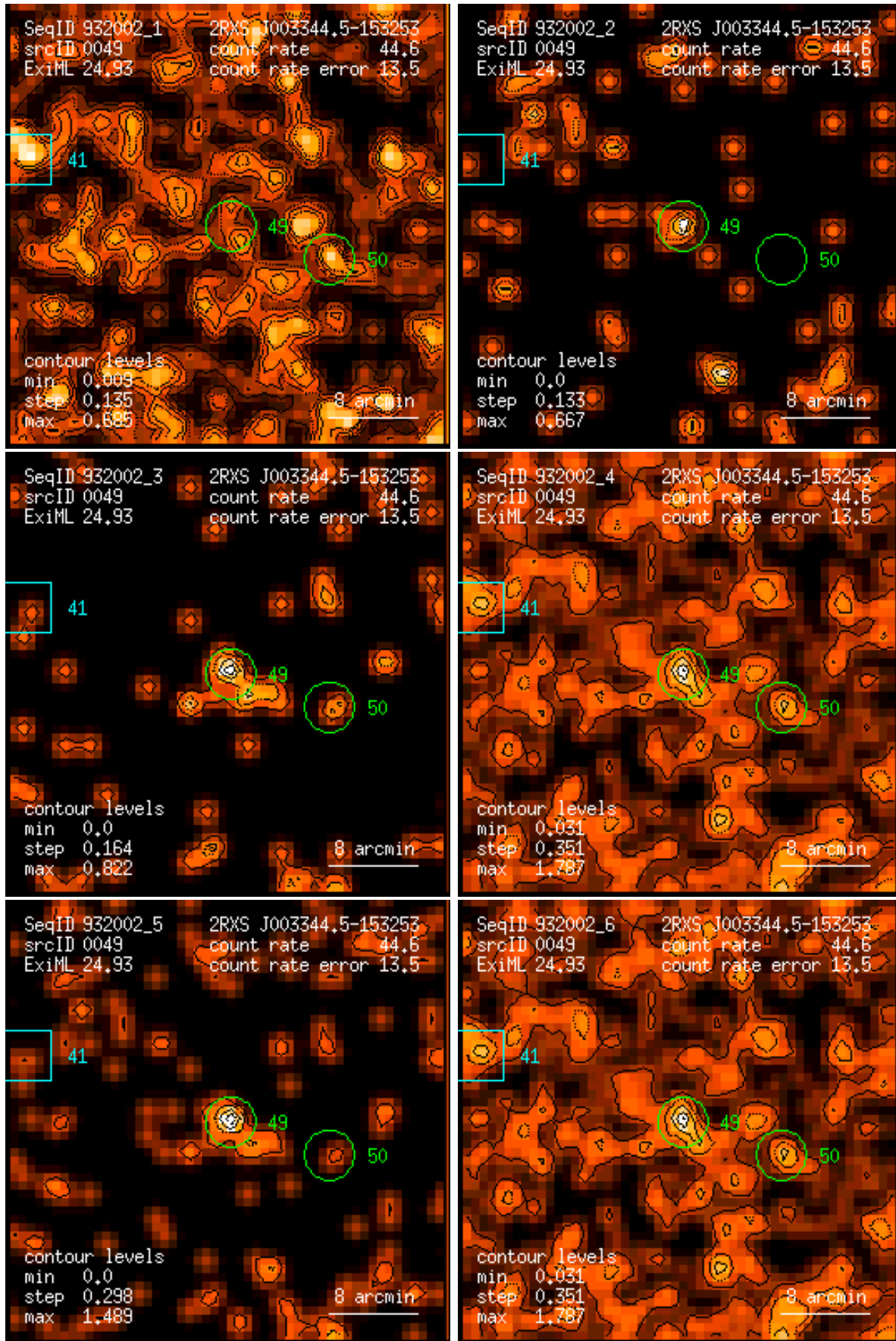
Figure 49: RASS 932002: detection 0049: band rate images, Gaussian filter: (1) PSPC channels 11 – 41, (2) 52 – 90, (3) 91 – 201, (4) 11 – 235, (5) 52 – 201, (6) 11 – 201. Broad band rates in counts/ks. Band rate contour levels in counts/ks/arcmin 2 .
