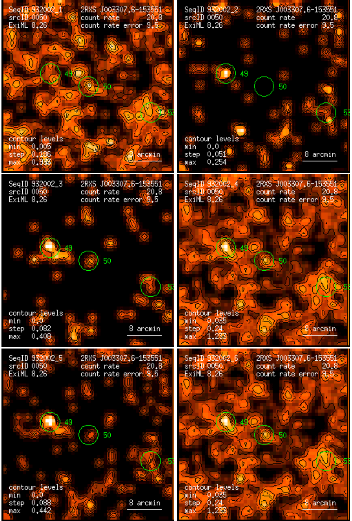
Figure 50: RASS 932002: detection 0050: band rate images, Gaussian filter: (1) PSPC channels 11 – 41, (2) 52 – 90, (3) 91 – 201, (4) 11 – 235, (5) 52 – 201, (6) 11 – 201. Broad band rates in counts/ks. Band rate contour levels in counts/ks/arcmin 2 .
