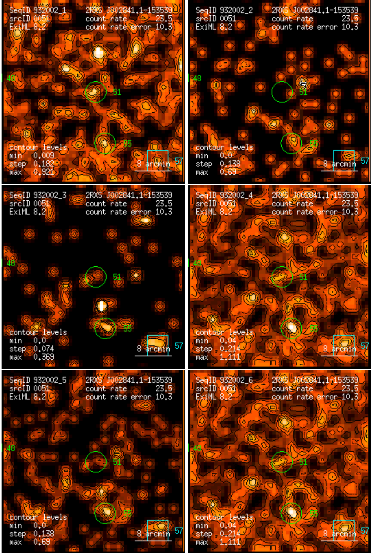
Figure 51: RASS 932002: detection 0051: band rate images, Gaussian filter: (1) PSPC channels 11 – 41, (2) 52 – 90, (3) 91 – 201, (4) 11 – 235, (5) 52 – 201, (6) 11 – 201. Broad band rates in counts/ks. Band rate contour levels in counts/ks/arcmin 2 .
