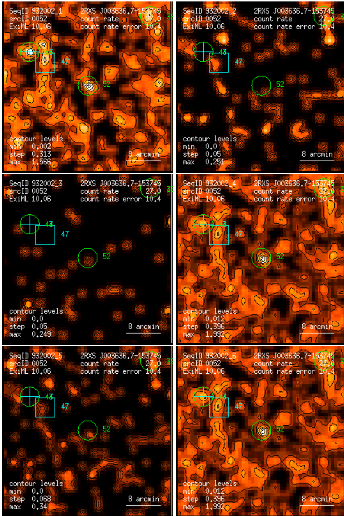
Figure 52: RASS 932002: detection 0052: band rate images, Gaussian filter: (1) PSPC channels 11 – 41, (2) 52 – 90, (3) 91 – 201, (4) 11 – 235, (5) 52 – 201, (6) 11 – 201. Broad band rates in counts/ks. Band rate contour levels in counts/ks/arcmin 2 .
