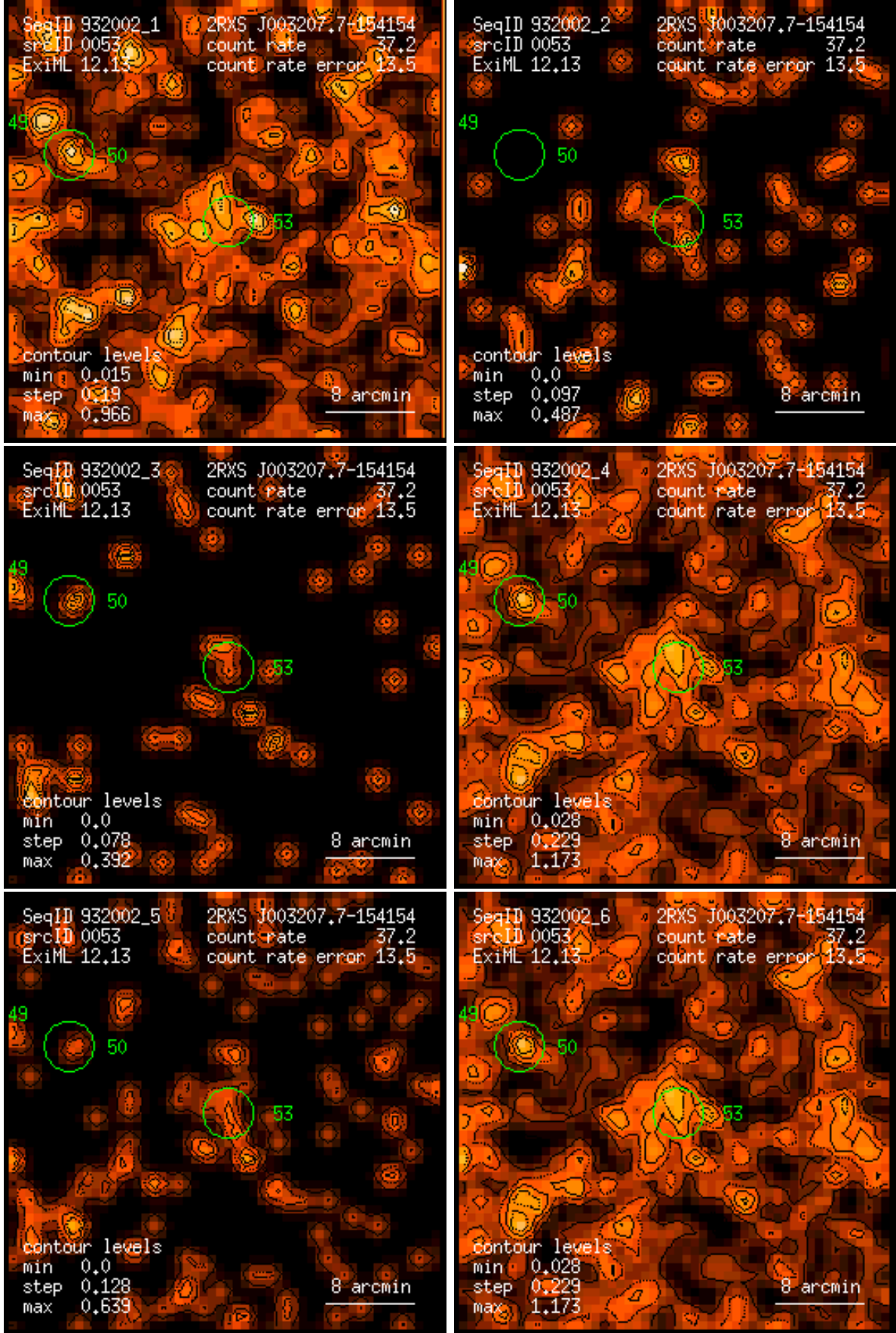
Figure 53: RASS 932002: detection 0053: band rate images, Gaussian filter: (1) PSPC channels 11 – 41, (2) 52 – 90, (3) 91 – 201, (4) 11 – 235, (5) 52 – 201, (6) 11 – 201. Broad band rates in counts/ks. Band rate contour levels in counts/ks/arcmin 2 .
