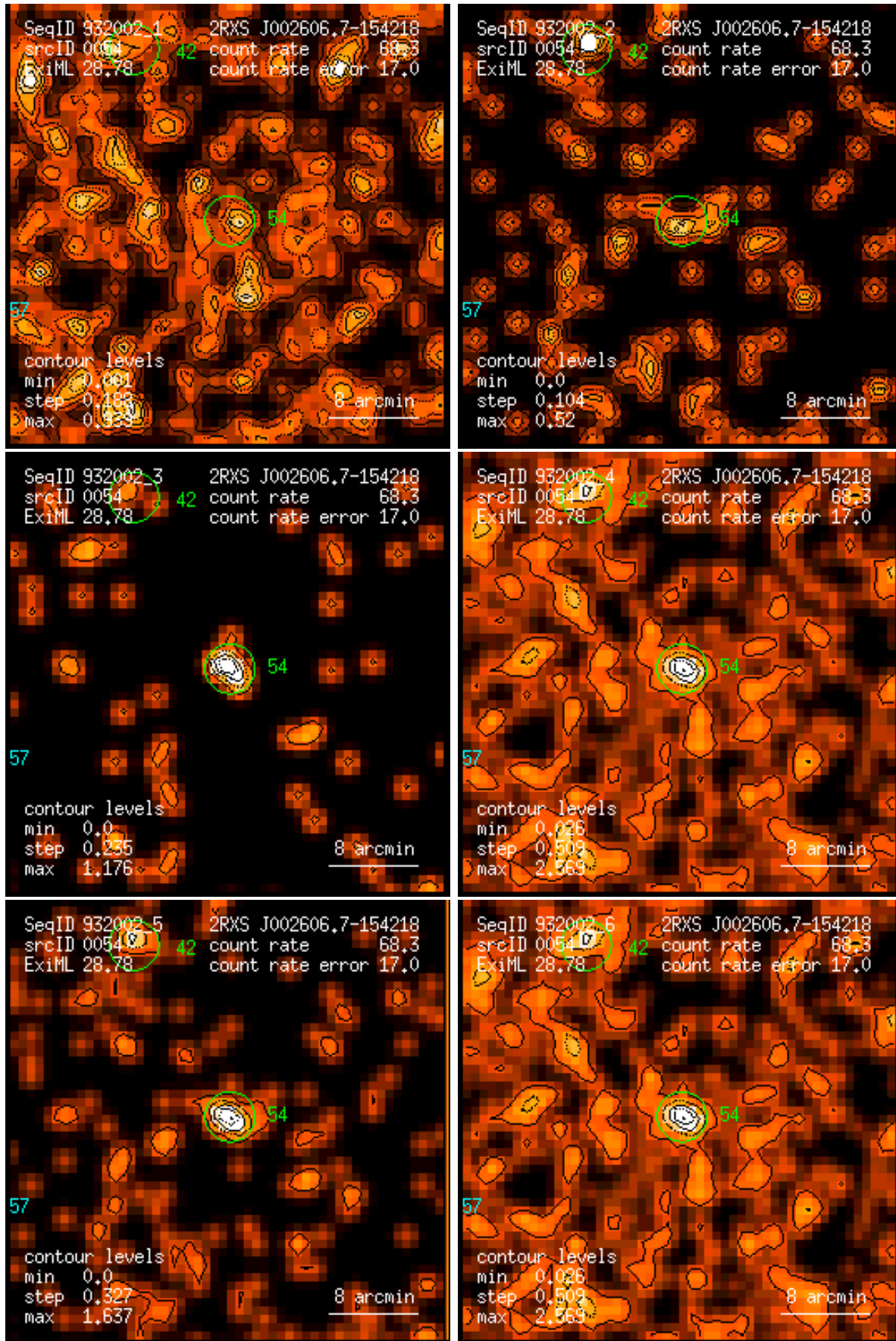
Figure 54: RASS 932002: detection 0054: band rate images, Gaussian filter: (1) PSPC channels 11 – 41, (2) 52 – 90, (3) 91 – 201, (4) 11 – 235, (5) 52 – 201, (6) 11 – 201. Broad band rates in counts/ks. Band rate contour levels in counts/ks/arcmin 2 .
