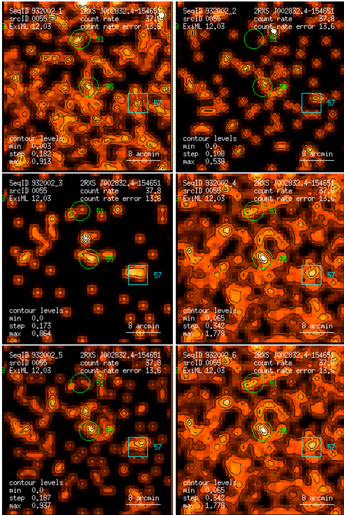
Figure 55: RASS 932002: detection 0055: band rate images, Gaussian filter: (1) PSPC channels 11 – 41, (2) 52 – 90, (3) 91 – 201, (4) 11 – 235, (5) 52 – 201, (6) 11 – 201. Broad band rates in counts/ks. Band rate contour levels in counts/ks/arcmin 2 .
