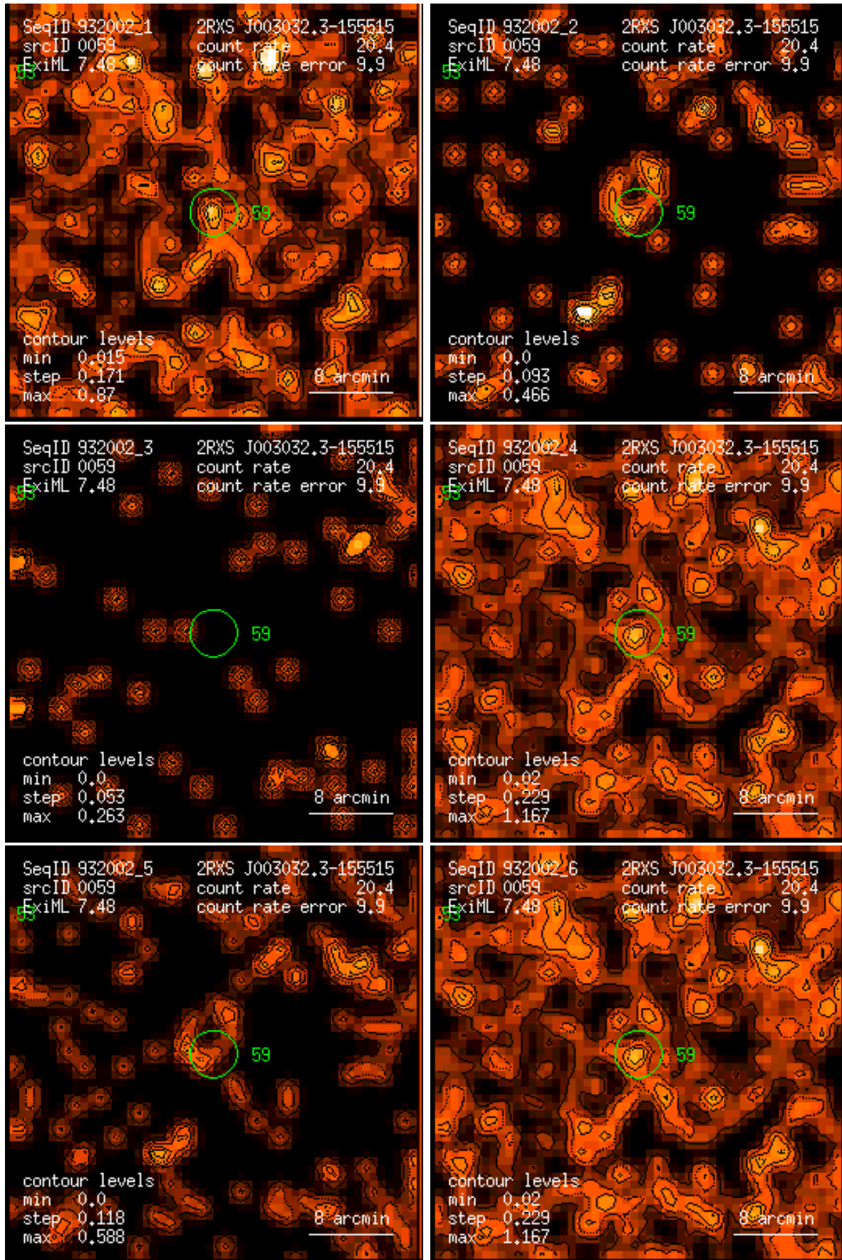
Figure 59: RASS 932002: detection 0059: band rate images, Gaussian filter: (1) PSPC channels 11 – 41, (2) 52 – 90, (3) 91 – 201, (4) 11 – 235, (5) 52 – 201, (6) 11 – 201. Broad band rates in counts/ks. Band rate contour levels in counts/ks/arcmin 2 .
