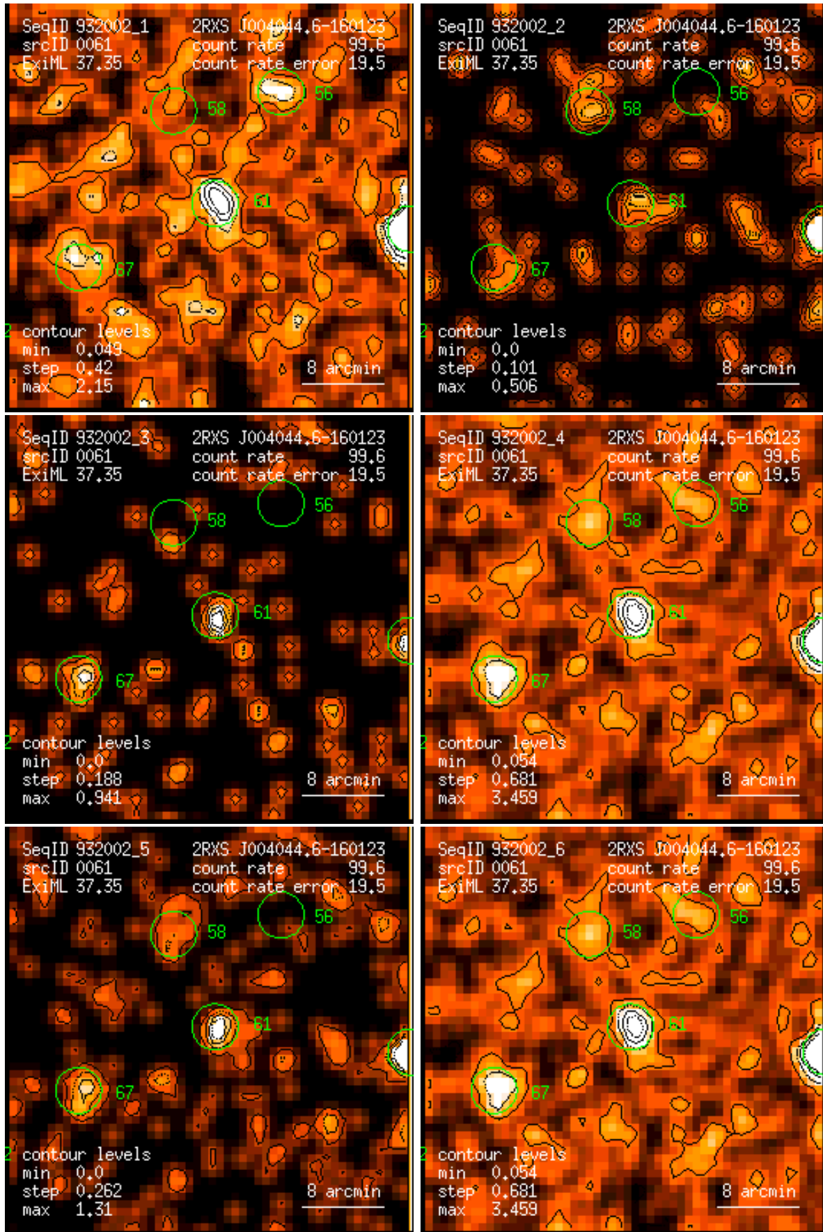
Figure 61: RASS 932002: detection 0061: band rate images, Gaussian filter: (1) PSPC channels 11 – 41, (2) 52 – 90, (3) 91 – 201, (4) 11 – 235, (5) 52 – 201, (6) 11 – 201. Broad band rates in counts/ks. Band rate contour levels in counts/ks/arcmin 2 .
