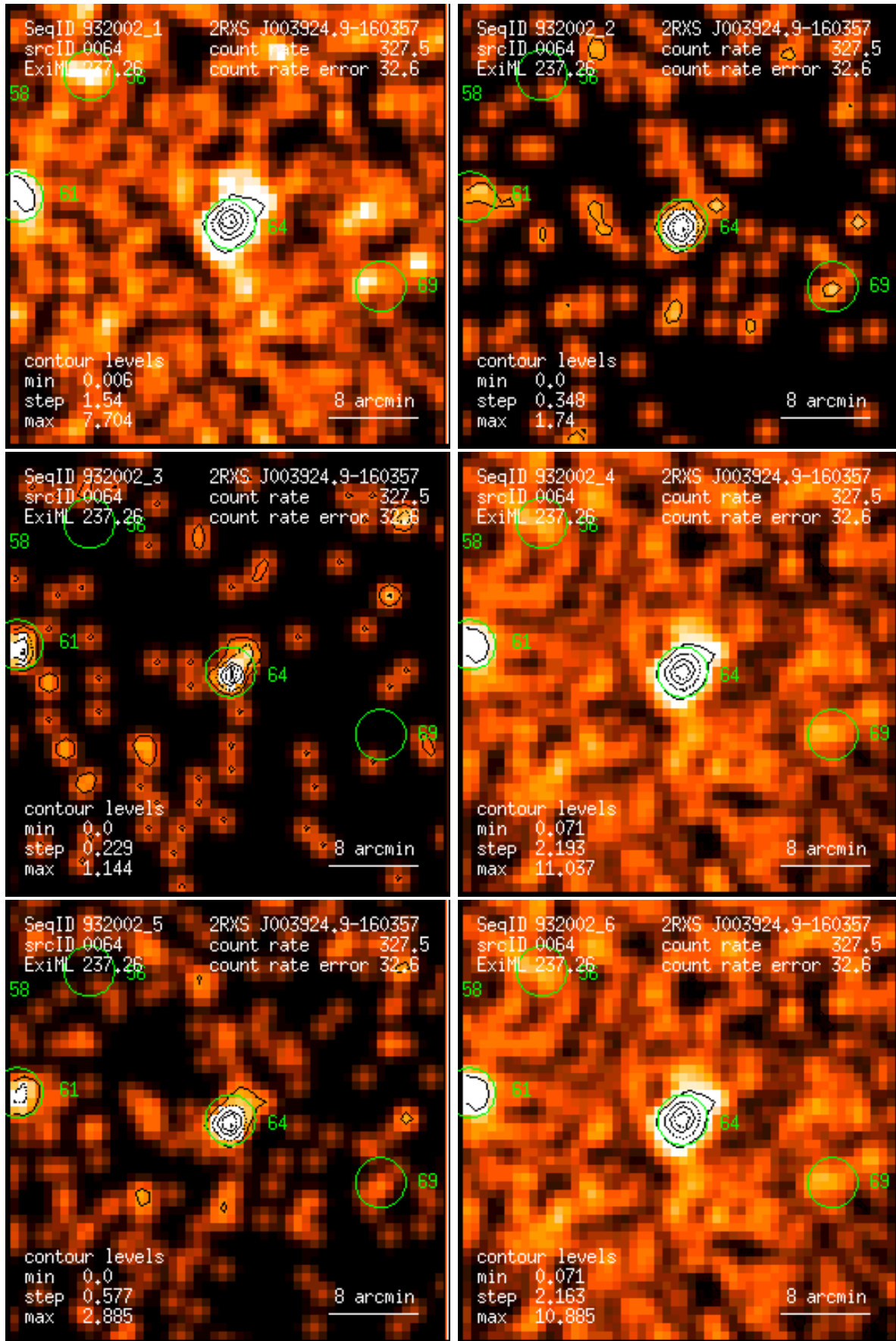
Figure 64: RASS 932002: detection 0064: band rate images, Gaussian filter: (1) PSPC channels 11 – 41, (2) 52 – 90, (3) 91 – 201, (4) 11 – 235, (5) 52 – 201, (6) 11 – 201. Broad band rates in counts/ks. Band rate contour levels in counts/ks/arcmin 2 .
