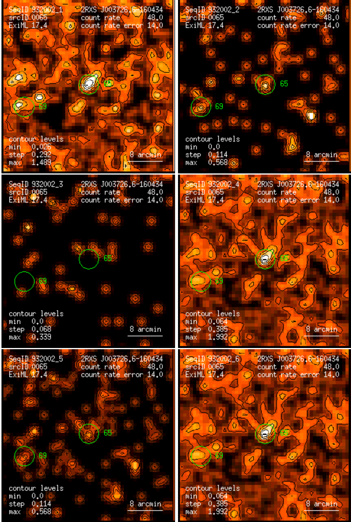
Figure 65: RASS 932002: detection 0065: band rate images, Gaussian filter: (1) PSPC channels 11 – 41, (2) 52 – 90, (3) 91 – 201, (4) 11 – 235, (5) 52 – 201, (6) 11 – 201. Broad band rates in counts/ks. Band rate contour levels in counts/ks/arcmin 2 .
