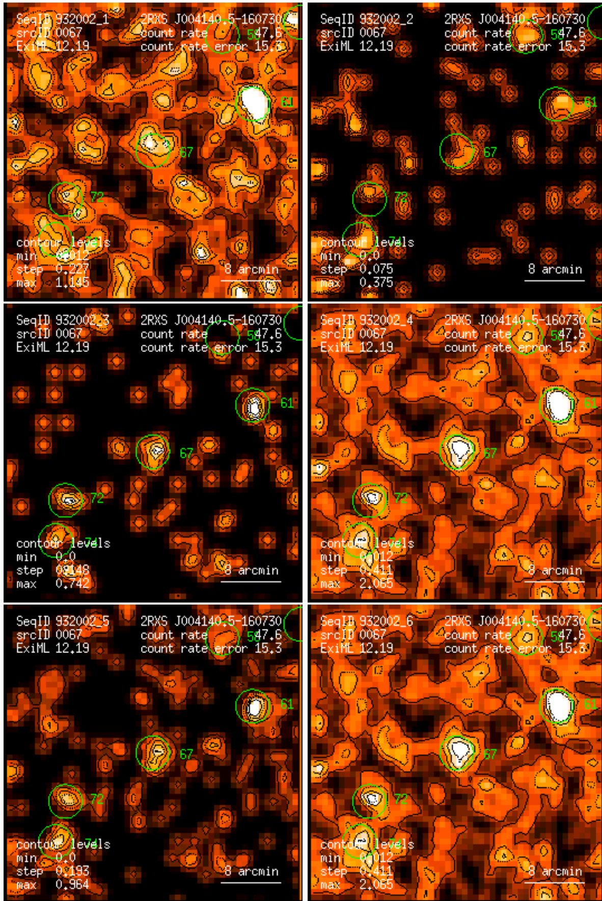
Figure 67: RASS 932002: detection 0067: band rate images, Gaussian filter: (1) PSPC channels 11 – 41, (2) 52 – 90, (3) 91 – 201, (4) 11 – 235, (5) 52 – 201, (6) 11 – 201. Broad band rates in counts/ks. Band rate contour levels in counts/ks/arcmin 2 .
