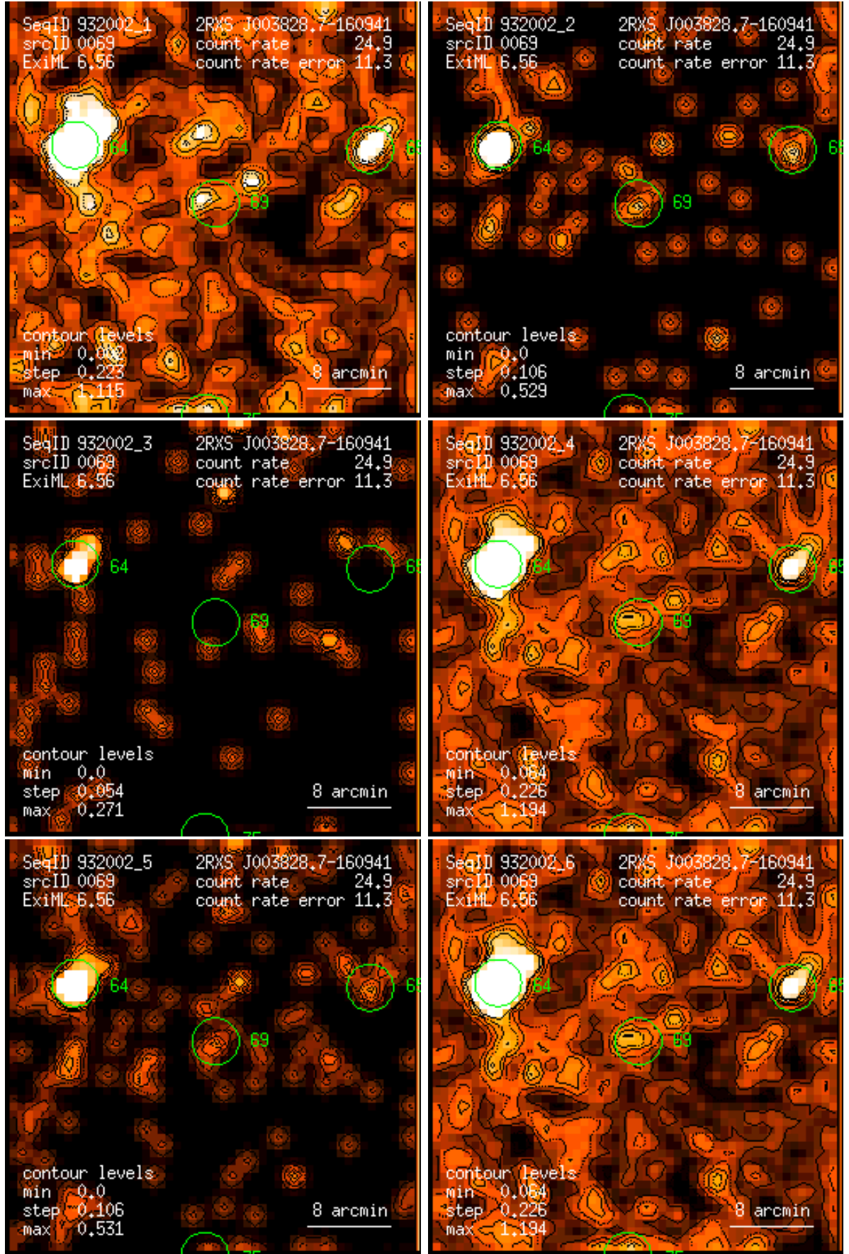
Figure 69: RASS 932002: detection 0069: band rate images, Gaussian filter: (1) PSPC channels 11 – 41, (2) 52 – 90, (3) 91 – 201, (4) 11 – 235, (5) 52 – 201, (6) 11 – 201. Broad band rates in counts/ks. Band rate contour levels in counts/ks/arcmin 2 .
