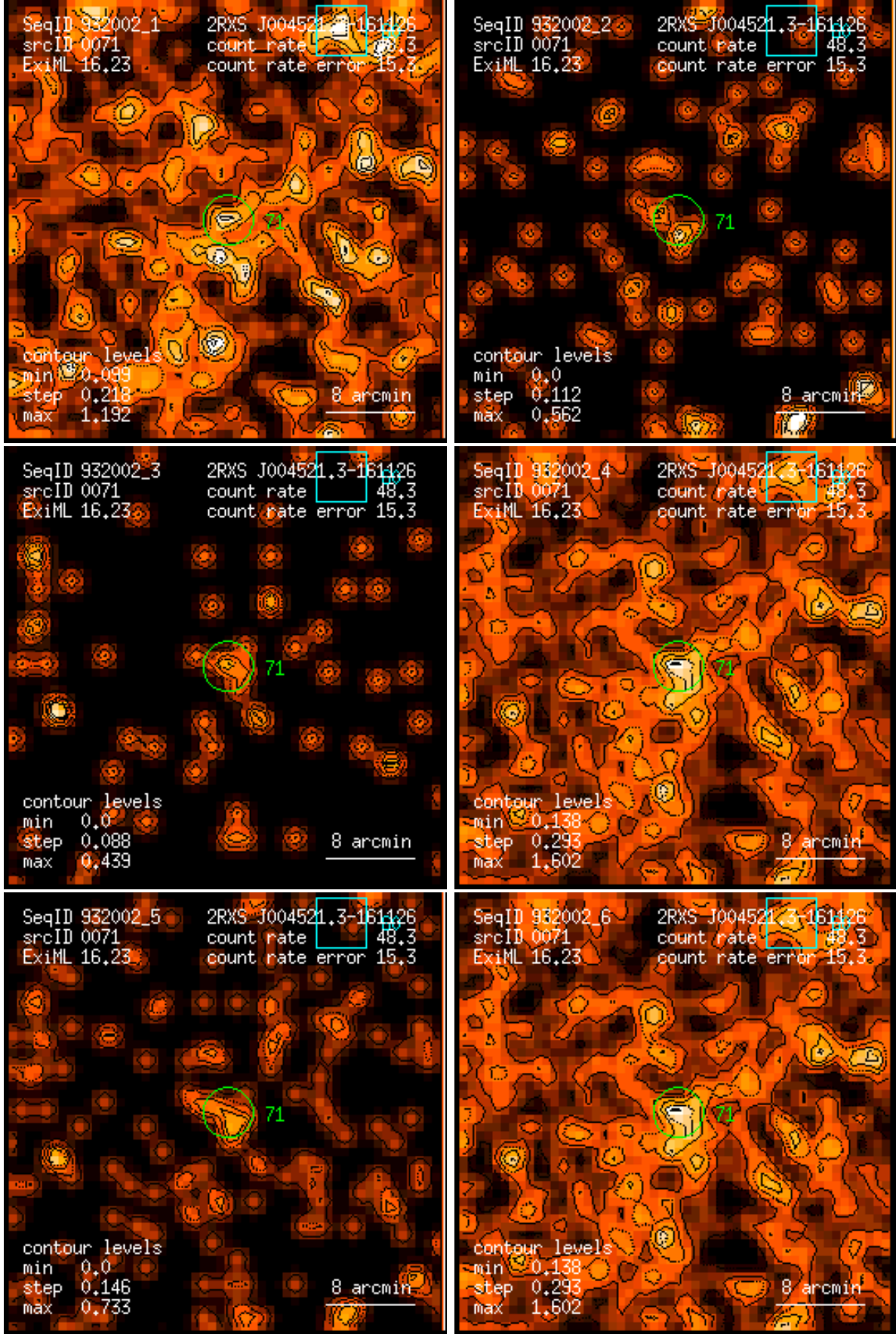
Figure 71: RASS 932002: detection 0071: band rate images, Gaussian filter: (1) PSPC channels 11 – 41, (2) 52 – 90, (3) 91 – 201, (4) 11 – 235, (5) 52 – 201, (6) 11 – 201. Broad band rates in counts/ks. Band rate contour levels in counts/ks/arcmin 2 .
