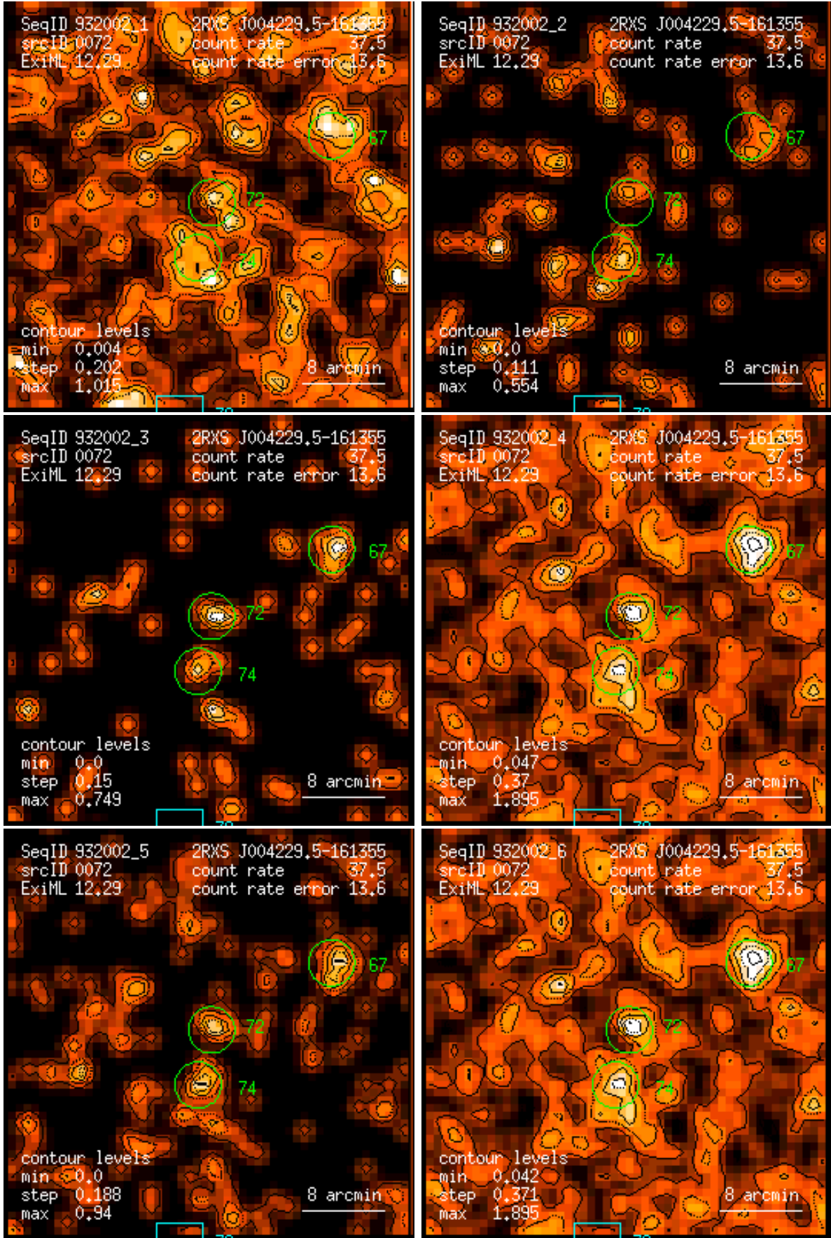
Figure 72: RASS 932002: detection 0072: band rate images, Gaussian filter: (1) PSPC channels 11 – 41, (2) 52 – 90, (3) 91 – 201, (4) 11 – 235, (5) 52 – 201, (6) 11 – 201. Broad band rates in counts/ks. Band rate contour levels in counts/ks/arcmin 2 .
