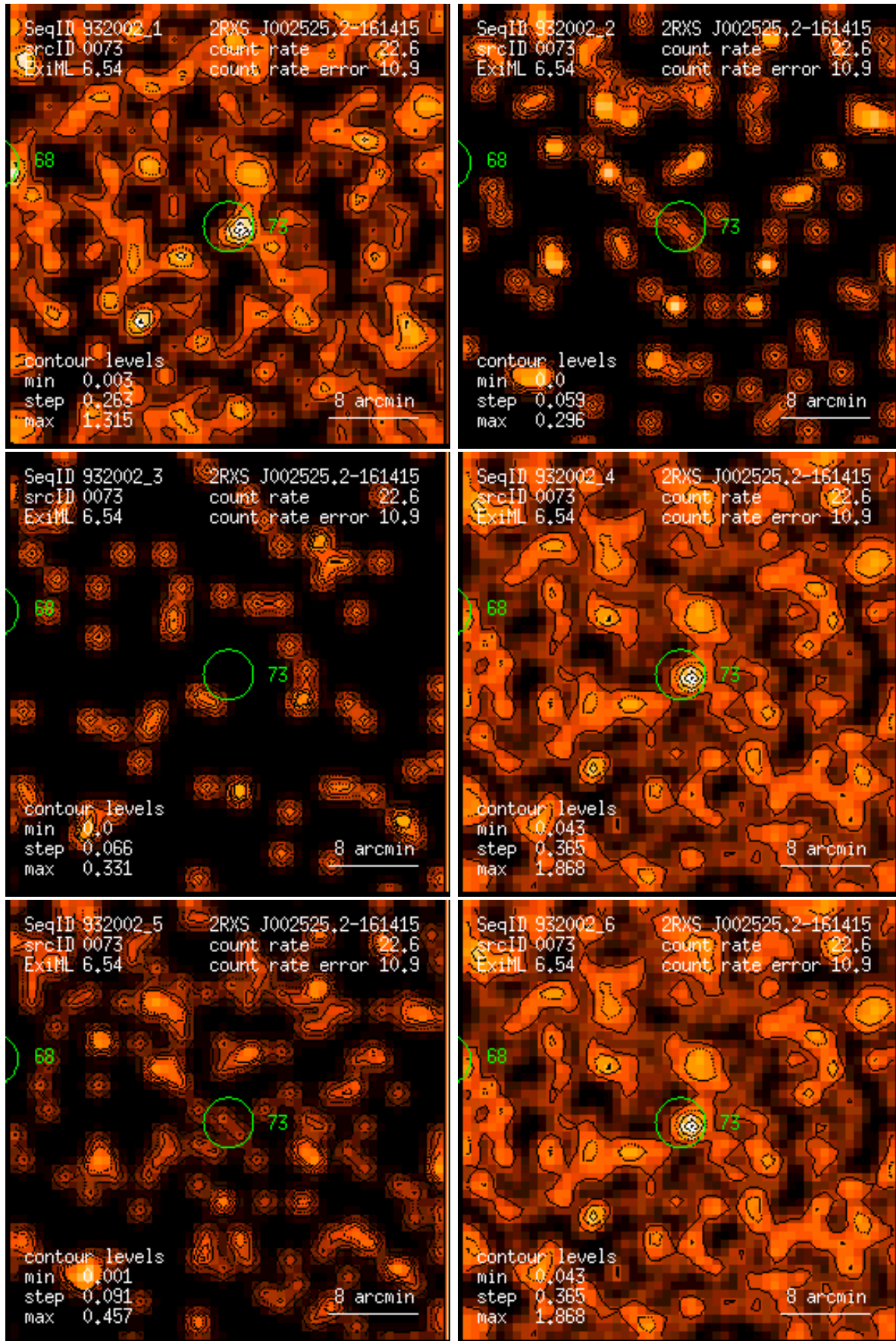
Figure 73: RASS 932002: detection 0073: band rate images, Gaussian filter: (1) PSPC channels 11 – 41, (2) 52 – 90, (3) 91 – 201, (4) 11 – 235, (5) 52 – 201, (6) 11 – 201. Broad band rates in counts/ks. Band rate contour levels in counts/ks/arcmin 2 .
