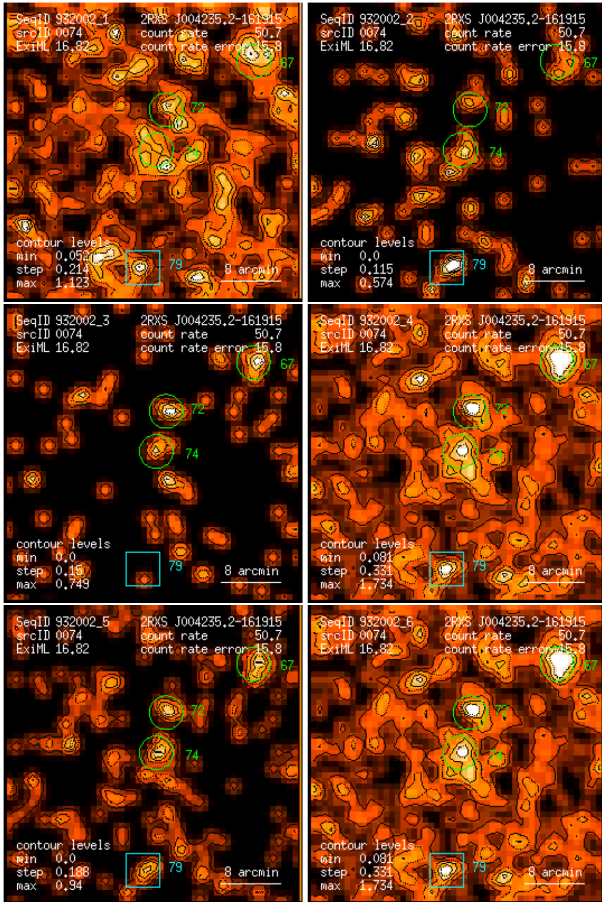
Figure 74: RASS 932002: detection 0074: band rate images, Gaussian filter: (1) PSPC channels 11 – 41, (2) 52 – 90, (3) 91 – 201, (4) 11 – 235, (5) 52 – 201, (6) 11 – 201. Broad band rates in counts/ks. Band rate contour levels in counts/ks/arcmin 2 .
