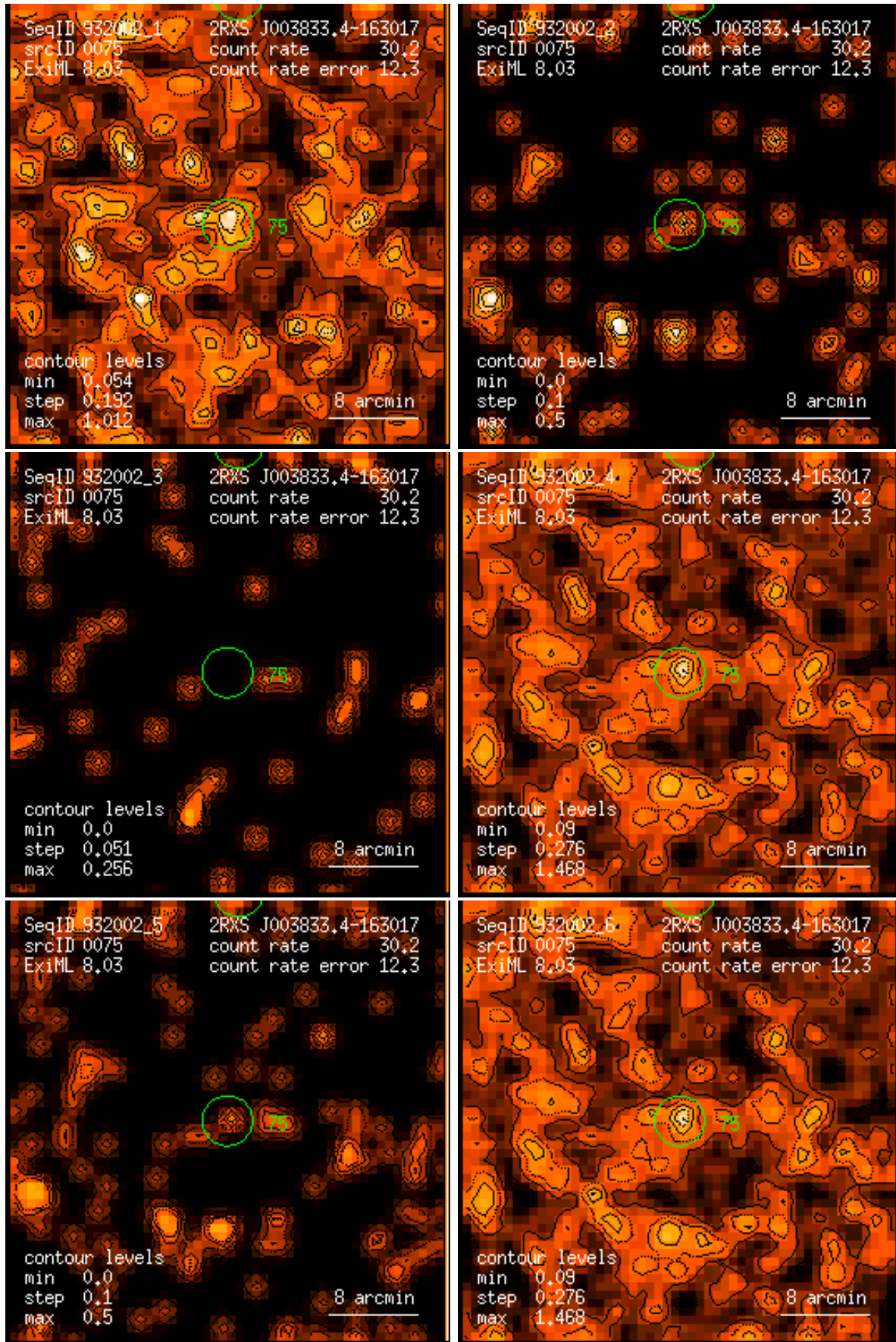
Figure 75: RASS 932002: detection 0075: band rate images, Gaussian filter: (1) PSPC channels 11 – 41, (2) 52 – 90, (3) 91 – 201, (4) 11 – 235, (5) 52 – 201, (6) 11 – 201. Broad band rates in counts/ks. Band rate contour levels in counts/ks/arcmin 2 .
