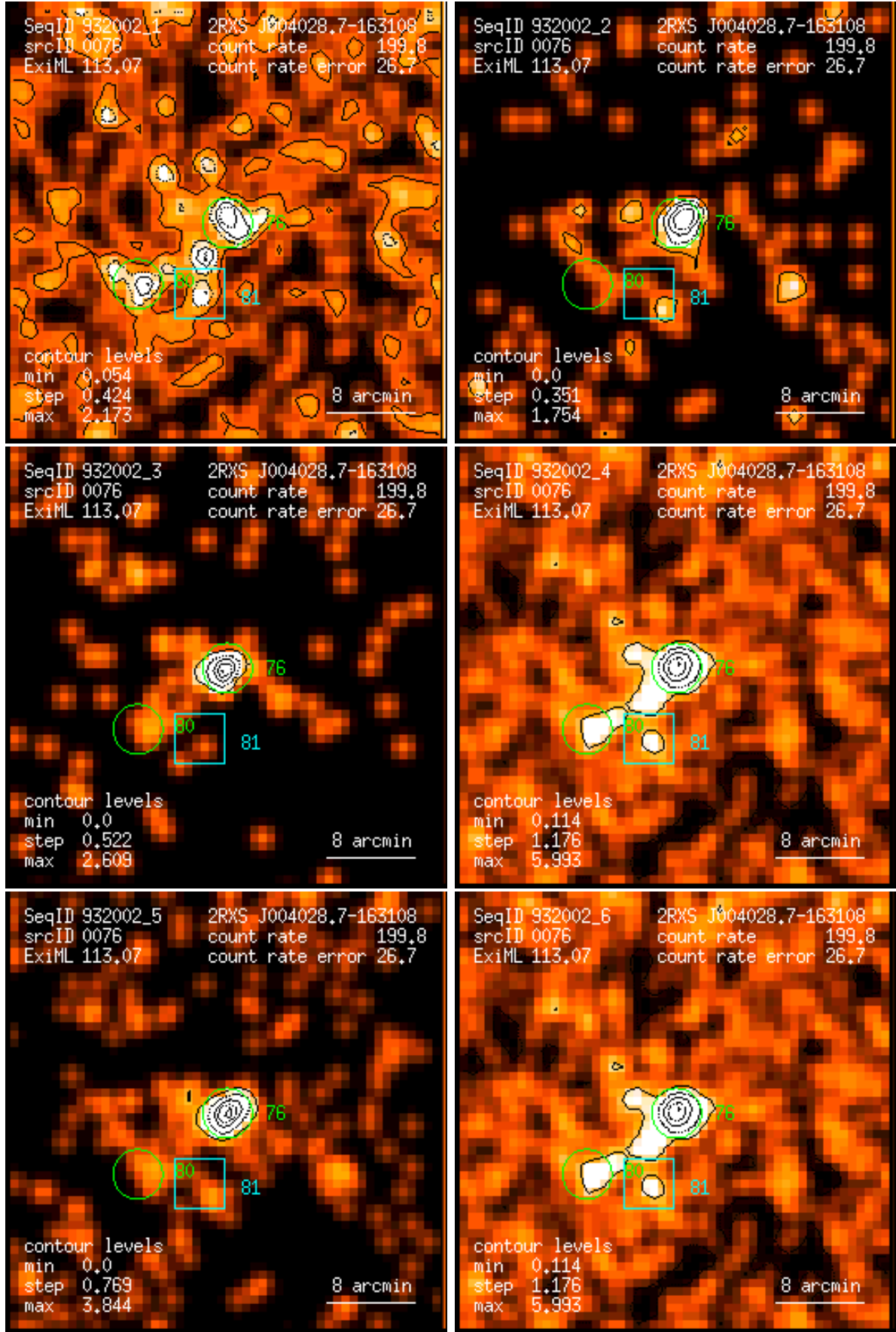
Figure 76: RASS 932002: detection 0076: band rate images, Gaussian filter: (1) PSPC channels 11 – 41, (2) 52 – 90, (3) 91 – 201, (4) 11 – 235, (5) 52 – 201, (6) 11 – 201. Broad band rates in counts/ks. Band rate contour levels in counts/ks/arcmin 2 .
