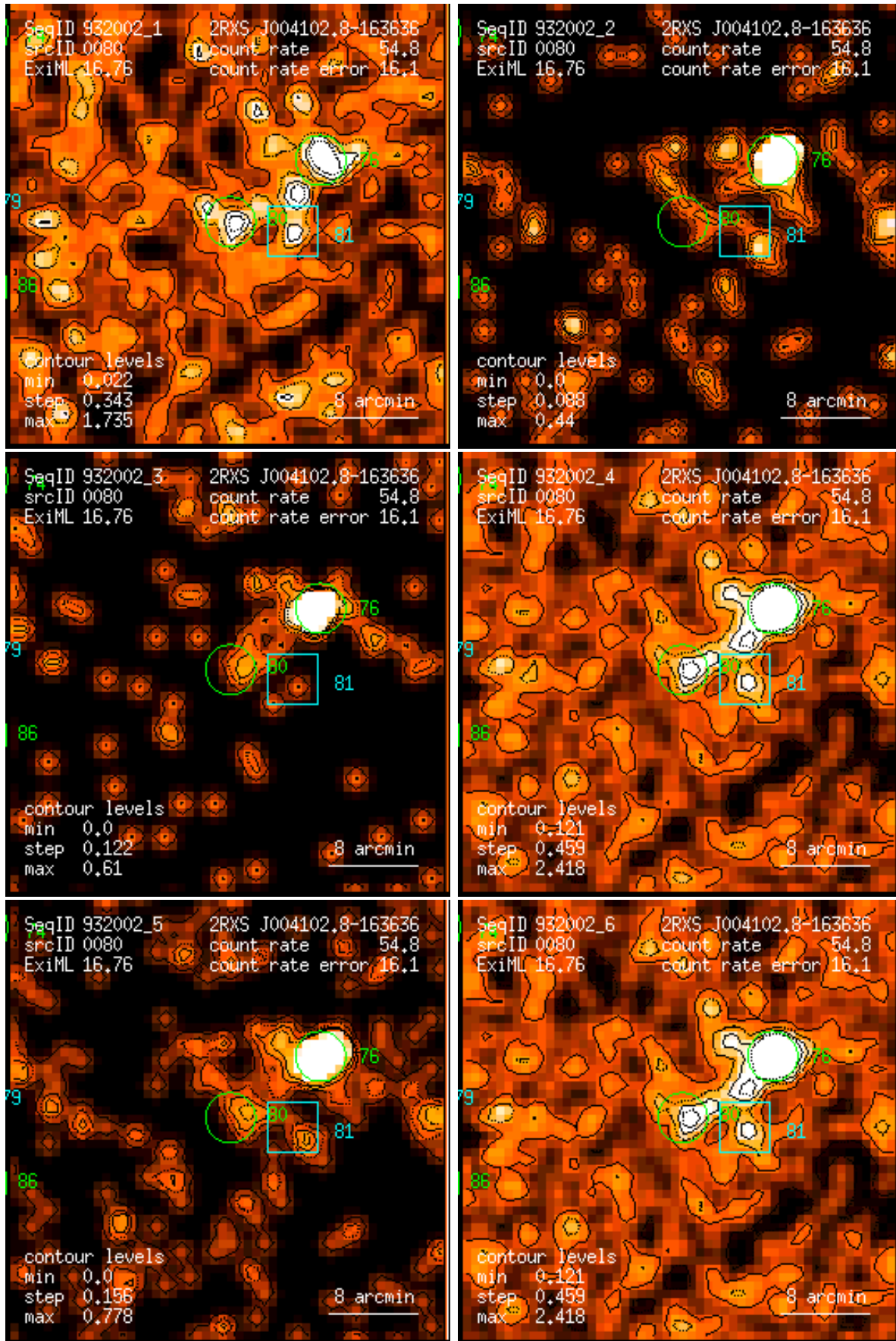
Figure 80: RASS 932002: detection 0080: band rate images, Gaussian filter: (1) PSPC channels 11 – 41, (2) 52 – 90, (3) 91 – 201, (4) 11 – 235, (5) 52 – 201, (6) 11 – 201. Broad band rates in counts/ks. Band rate contour levels in counts/ks/arcmin 2 .
