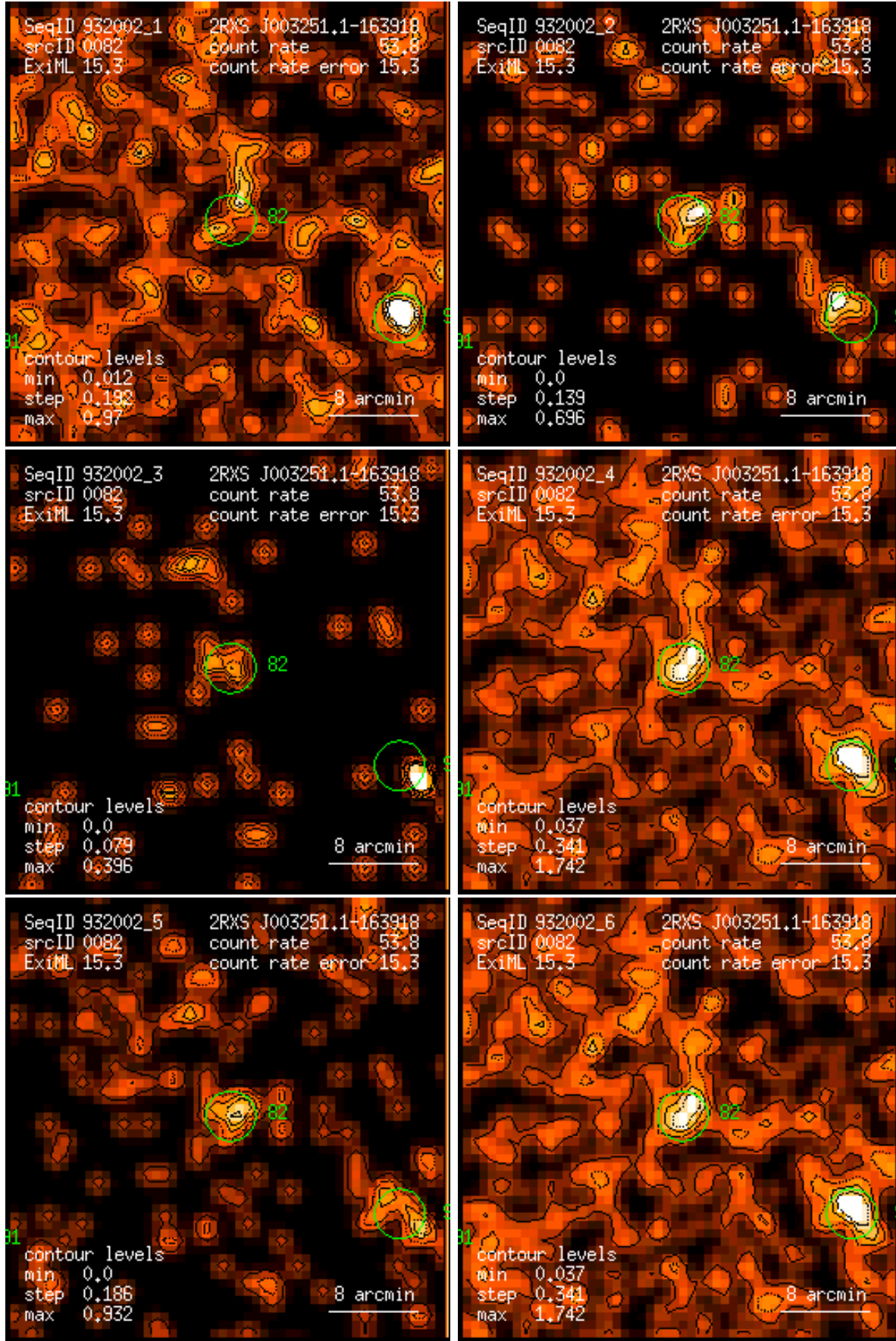
Figure 82: RASS 932002: detection 0082: band rate images, Gaussian filter: (1) PSPC channels 11 – 41, (2) 52 – 90, (3) 91 – 201, (4) 11 – 235, (5) 52 – 201, (6) 11 – 201. Broad band rates in counts/ks. Band rate contour levels in counts/ks/arcmin 2 .
