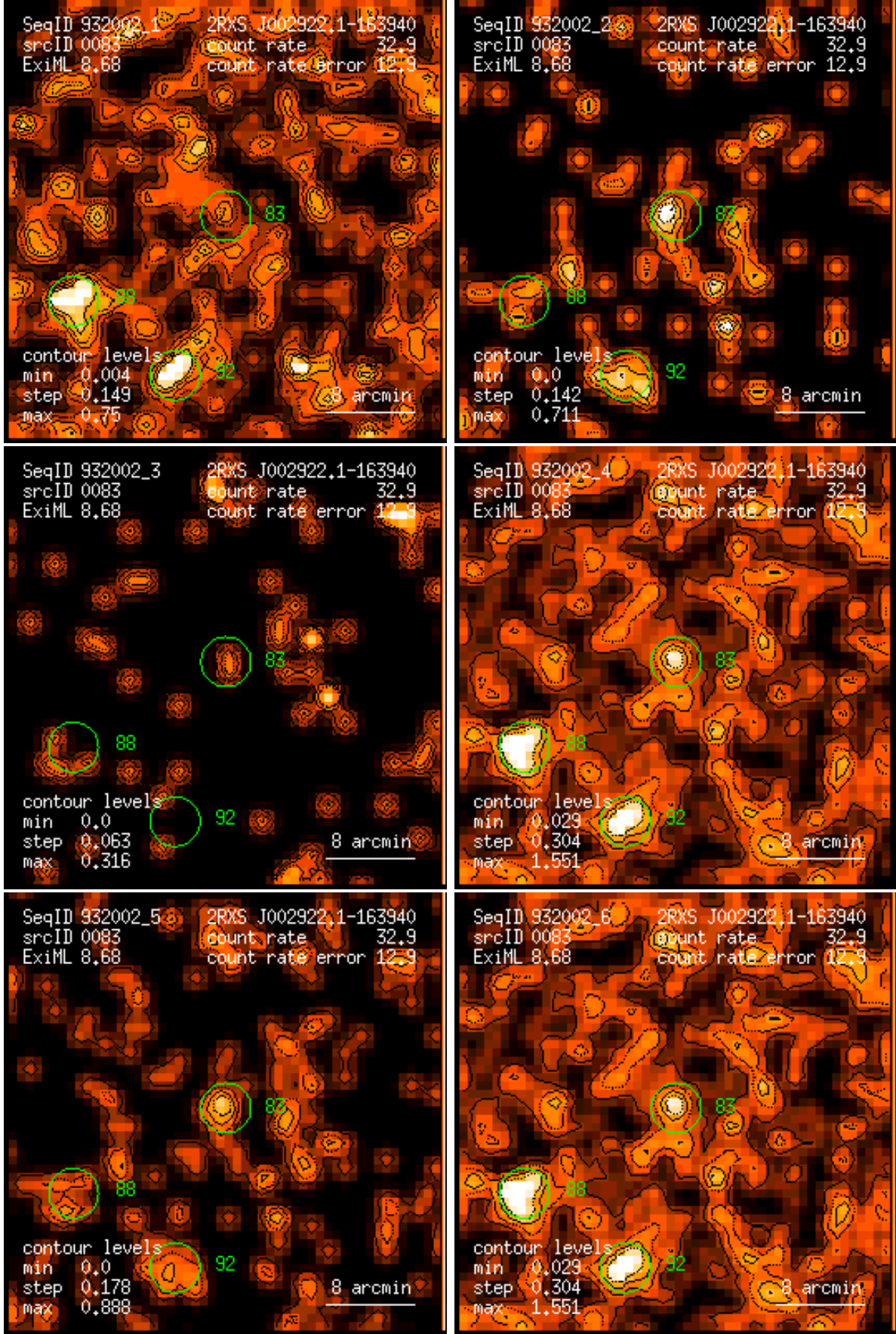
Figure 83: RASS 932002: detection 0083: band rate images, Gaussian filter: (1) PSPC channels 11 – 41, (2) 52 – 90, (3) 91 – 201, (4) 11 – 235, (5) 52 – 201, (6) 11 – 201. Broad band rates in counts/ks. Band rate contour levels in counts/ks/arcmin 2 .
