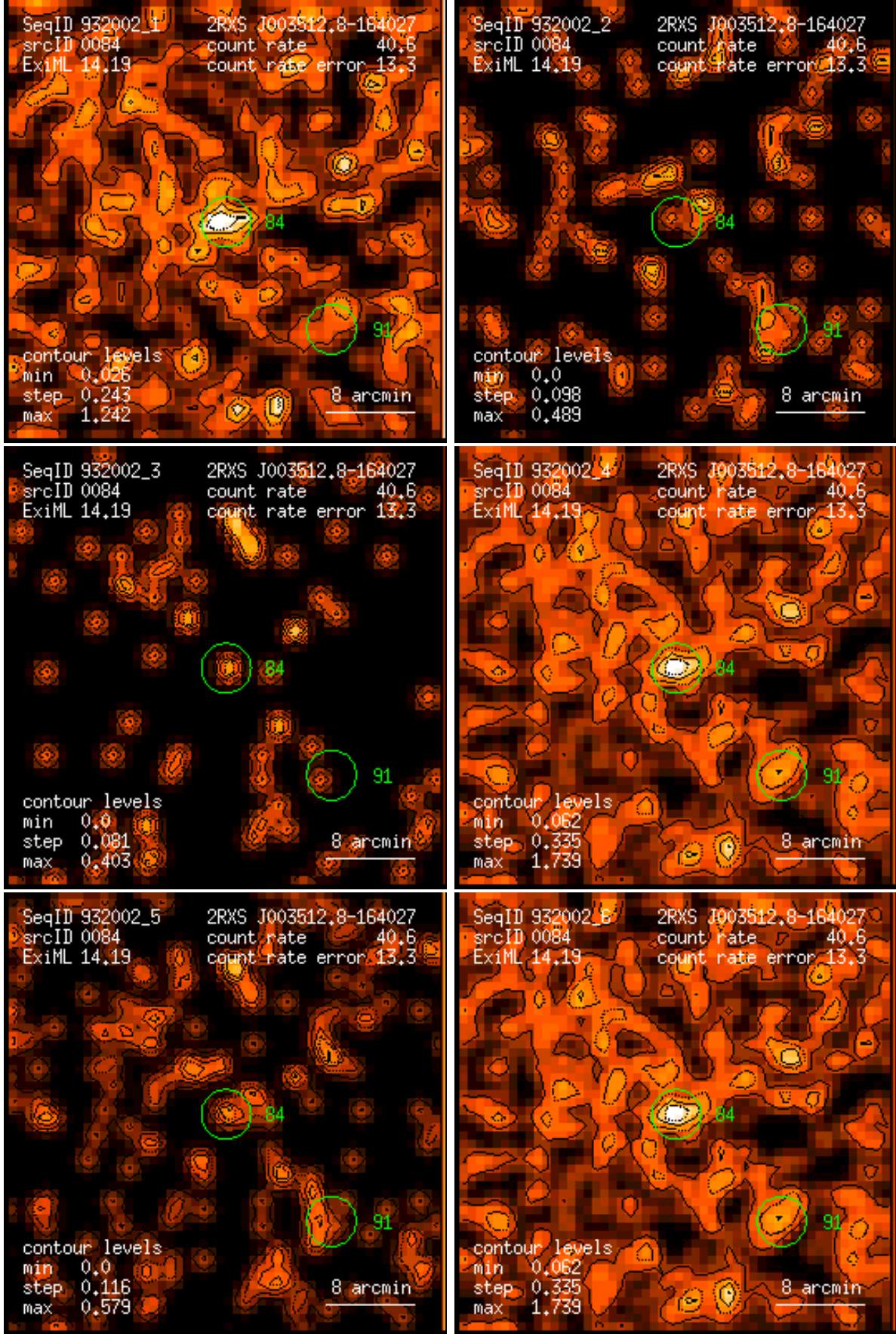
Figure 84: RASS 932002: detection 0084: band rate images, Gaussian filter: (1) PSPC channels 11 – 41, (2) 52 – 90, (3) 91 – 201, (4) 11 – 235, (5) 52 – 201, (6) 11 – 201. Broad band rates in counts/ks. Band rate contour levels in counts/ks/arcmin 2 .
